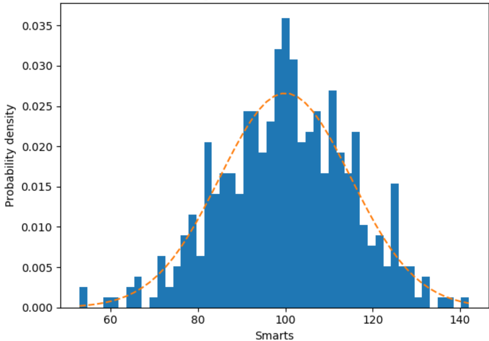
Histogram of IQ: \mu = 100, \sigma = 15
