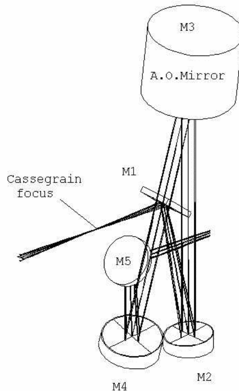
Figure 12: Main optics
