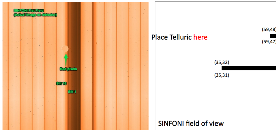
Figure 8: Left: This is a SINFONI Flat Field image. The disc of bad pixels near the centre of the detector falls on slit #16, which crosses the centre of the field of view of SINFONI. Right: This is the reconstructed FOV of SINFONI, showing the location of the blind spots. Slit #16 corresponds to y=31 and 32 . Slit #24 corresponds on y=47 and 48 .
