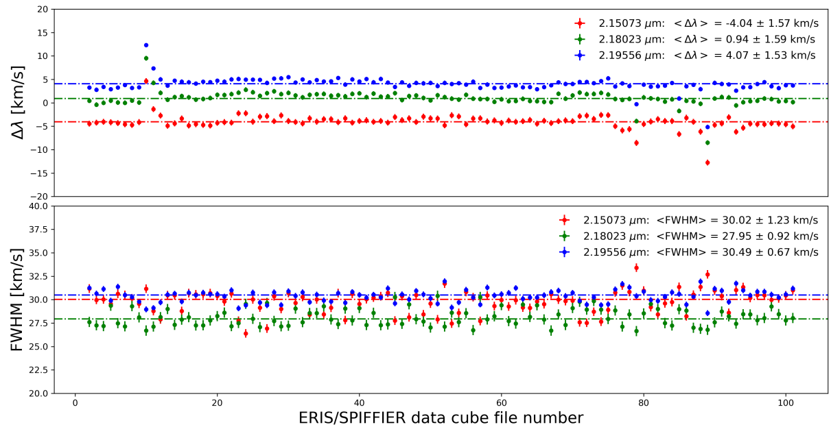
Figure 1: the wavelength shift (top panel) and FWHM (bottom panel) for three [OH] lines, as measured in a sample of 100 ERIS/SPIFFIER data cubes in K_{\text{middle}}/100\text{mas} . These observations were made in a wide variety of pointings (i.e. the full range of accessible altitudes and instrument rotator angles).
