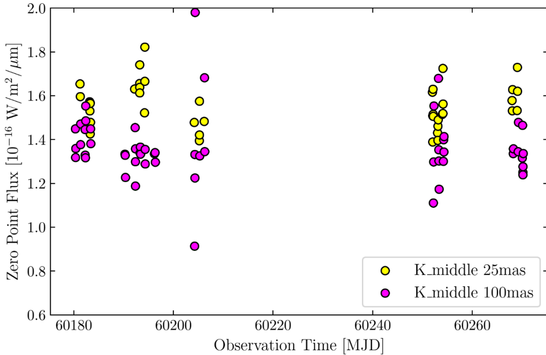
Figure 2: the variation of the zero point flux as derived from 100 standard stars taken between August and November 2023. The scatter is partly due to varying photometric and seeing conditions.
