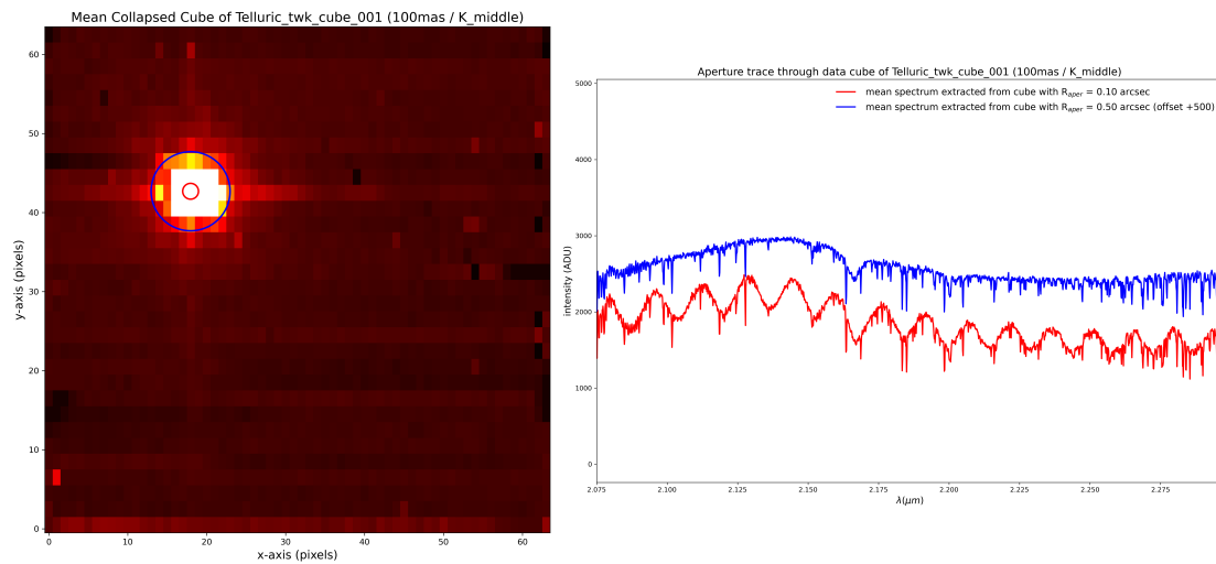
Figure 3: an example of extracted spectrum “wiggles” in an under-sampled ERIS/SPIFFIER standard star. Being under-sampled, the majority of the stand star’s flux falls into a single rectangular spaxel. When extracting through the data cube over an aperture close to this single pixel (the red aperture in the collapsed cube shown on the left), the undulating spectrum becomes apparent (red trace: right-hand panel). When extracted over a reasonable aperture (blue aperture), the under-sampled wiggles average out (blue trace offset by 500 ADU).
