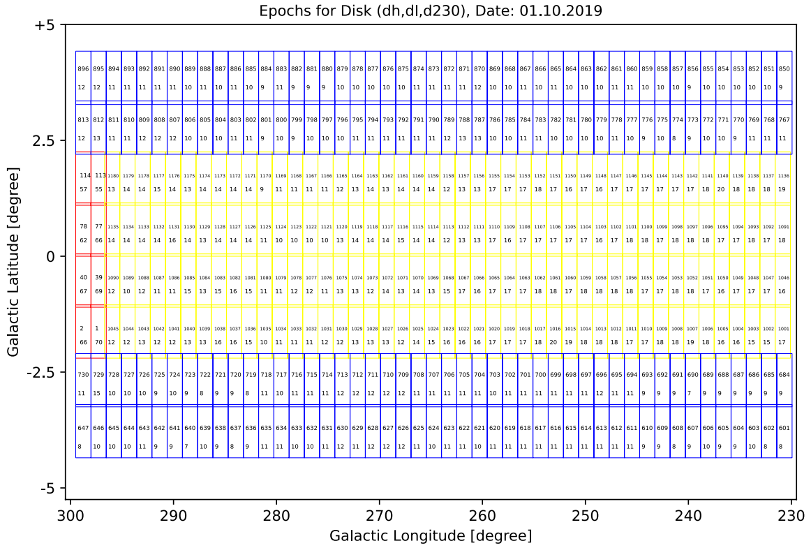
Figure 1(a-c). Maps of the cumulative sky coverage in VVVX DR1 and DR2 and the number of Ks epochs for each tile, including data from the earlier VVV survey. In each tile, the lower number is the number of Ks epochs and the upper number is the unique tile ID number. The new VVVX fields are coloured green, blue and yellow and the original VVV area is coloured red. A few additional epochs per tile were also obtained in the original VVV area.
