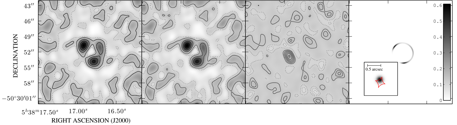
FIG. 6.— The best fit lens model for SPT0538-50 using a single source component, for comparison with Figure 4. Left to right are the “dirty” image, the model dirty image, the difference between data and model, and the full-resolution source model. Contours in the two panels on the left start at \pm 2 times the rms noise in the residual map ( \sigma ), increasing in steps of 10\sigma , while contours in the third panel increase in steps of \pm 1\sigma . The peak in the residual map has a significance of >5\sigma . As shown in Figure 4, a second source component completely eliminates this high peak and has a significance >10\sigma in the visibility space.
