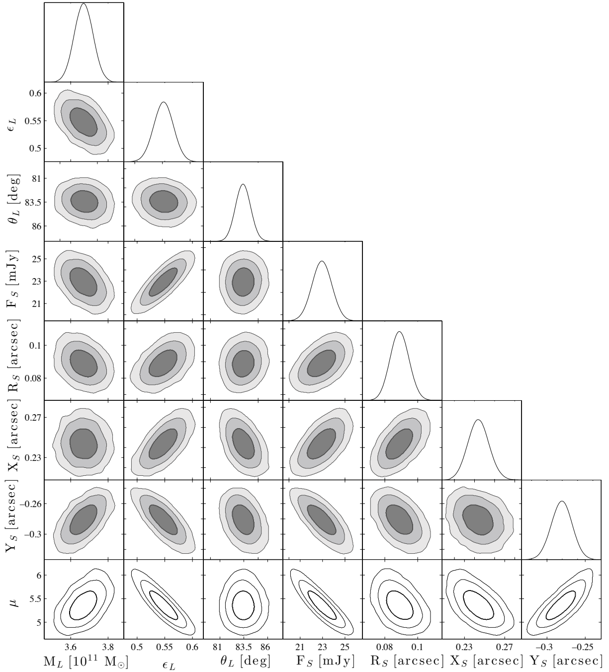
FIG. 3.— Parameter degeneracy plot for SPT0346-52, a representative example of the model uncertainties. Some nuisance parameters are not shown. Marginalized distributions for each parameter along the bottom axis are shown as histograms on the diagonal. The bottom row shows correlations between \mu , which is derived from the model and not a fit parameter, and the model parameters. The contours show the 1, 2, and 3 \sigma confidence regions.
