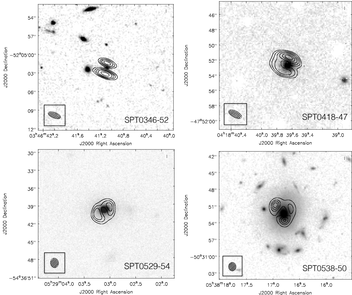
FIG. 1.— ALMA 350 GHz CLEANed images of the lensed DSGs (contours), on top of NIR imaging of the galaxy field (greyscale) from Hubble Space Telescope , VLT, and SOAR. Left to right they are SPT0346-52 ( HST ) and SPT0418-47 (VLT) in the top row and SPT0529-54 (SOAR) and SPT0538-50 ( HST ) in the bottom row. The ALMA contours begin at 5\sigma , increasing in steps of 10\sigma in the top left and bottom right images, and 5\sigma in the other two, as in Figure 4. The synthesized beam is shown in the lower left of each image. The HST images are a composite of the F110W and F160W filters, the VLT images are K band from ISAAC, and the SOAR image is K band from OSIRIS.
