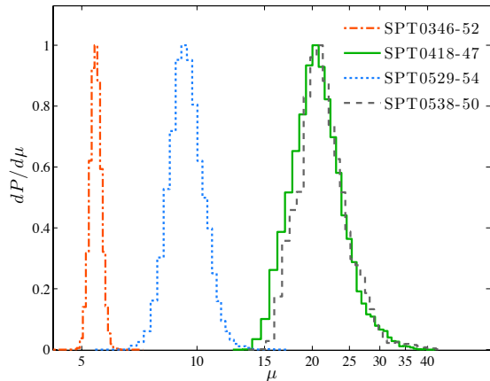
FIG. 5.— The source magnification distributions derived from the lens models. In the case of SPT0538-50, the total magnification of the two source-plane components is shown.
