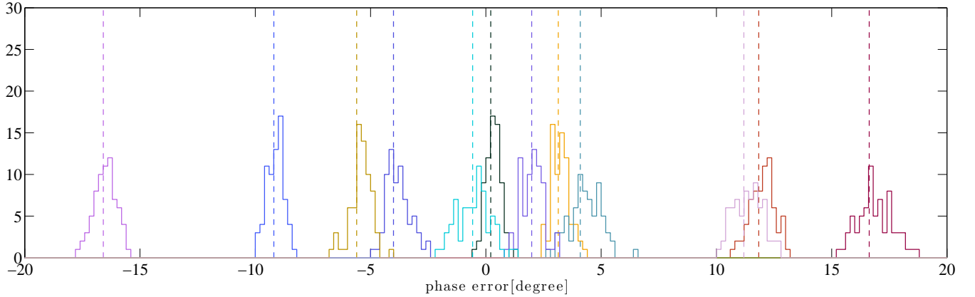
FIG. 8.— Antenna phase errors recovered in 70 simulated observations of a lens model with different noise realizations. Phase errors were introduced to the antennas, with values indicated by the vertical dashed lines. The histograms show the phase values recovered in fits to the simulated visibilities following the technique outlined here.
