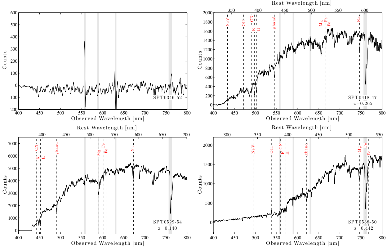
FIG. 2.— Optical spectra of the foreground lenses, from the VLT. The positions of major lines are marked by thin dashed lines. Sky lines are marked with grey shaded regions.
