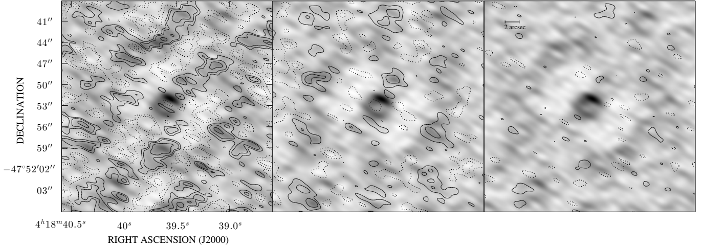
FIG. 7.— A comparison of image residuals for three different corrections to the antenna phases. The dirty image of SPT0418-47 is shown in greyscale beneath each panel. Contours show the image residuals after the source model is subtracted from the dirty image. Left: Residual structure after the model that fits the raw data (no self-calibration) best is subtracted from the data. Middle: The same, but for data calibrated using a CLEAN-based self-calibration. Right: The same, but for data calibrated using the procedure described in this work. The presence of residual structure away from the source, with no corresponding residual at the source position, is a clear sign of imperfectly corrected phase in the left two panels.
