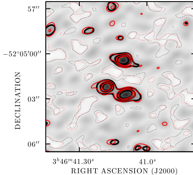
FIG. 9.— A comparison of the model proposed for SPT0346-52 from the low-resolution observations presented above and the higher-resolution observations obtained after submission. The “dirty” image of the extended configuration observations are shown in greyscale and black contours. The red contours are the predicted appearance given the model of Figure 4 and the uv sampling of the new data. Contours are drawn at \times 5 (dashed) and \times 20, 40, 60 (solid) times the rms noise.
