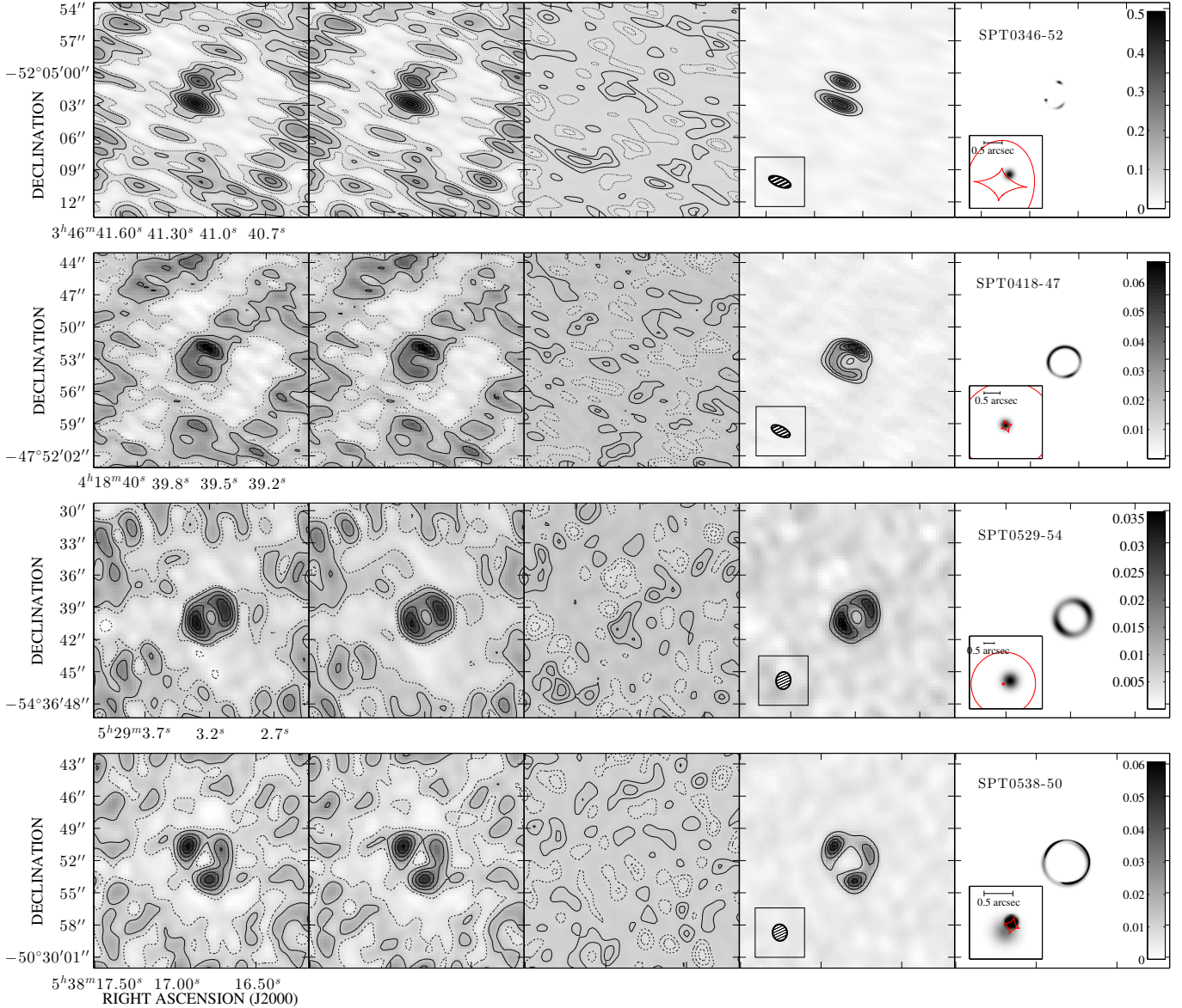
FIG. 4.— Modeling of the observed submillimeter emission. In each row, the panels from left to right are: the “dirty” image, model dirty image, residuals after subtraction, CLEANed image, and fully resolved lens model. Contours in the left two columns start at \pm 3 times the rms noise in the residual map (third column) and increase in steps of 10 times the rms noise, except in the second row where they increase in steps of 5 times the rms noise. Contours in the residuals are \pm 1, 2, \text{etc.} , times the rms noise, which is (top to bottom) 1.5, 1.7, 1.0, and 1.0 mJy. The contours in the CLEANed images start at 5\sigma and increase in levels of 10\sigma for the top and bottom rows and 5\sigma in the two middle rows. The apparently high significance structure in the dirty maps away from the source is due to the sidelobes of the synthesized (or “dirty”) beam, and should therefore be reproduced by the model in the second panel. The insets in the last panels show a magnified view of the positions of the emission in the source plane (greyscale) relative to the lensing caustics (red). In the source model for SPT0538-50 the greyscale is truncated at 10% of the peak intensity to make the second source component visible. The intensity scale for the right panel, in \text{Jy arcsec}^{-2} , is given by the colorbar in each figure.
