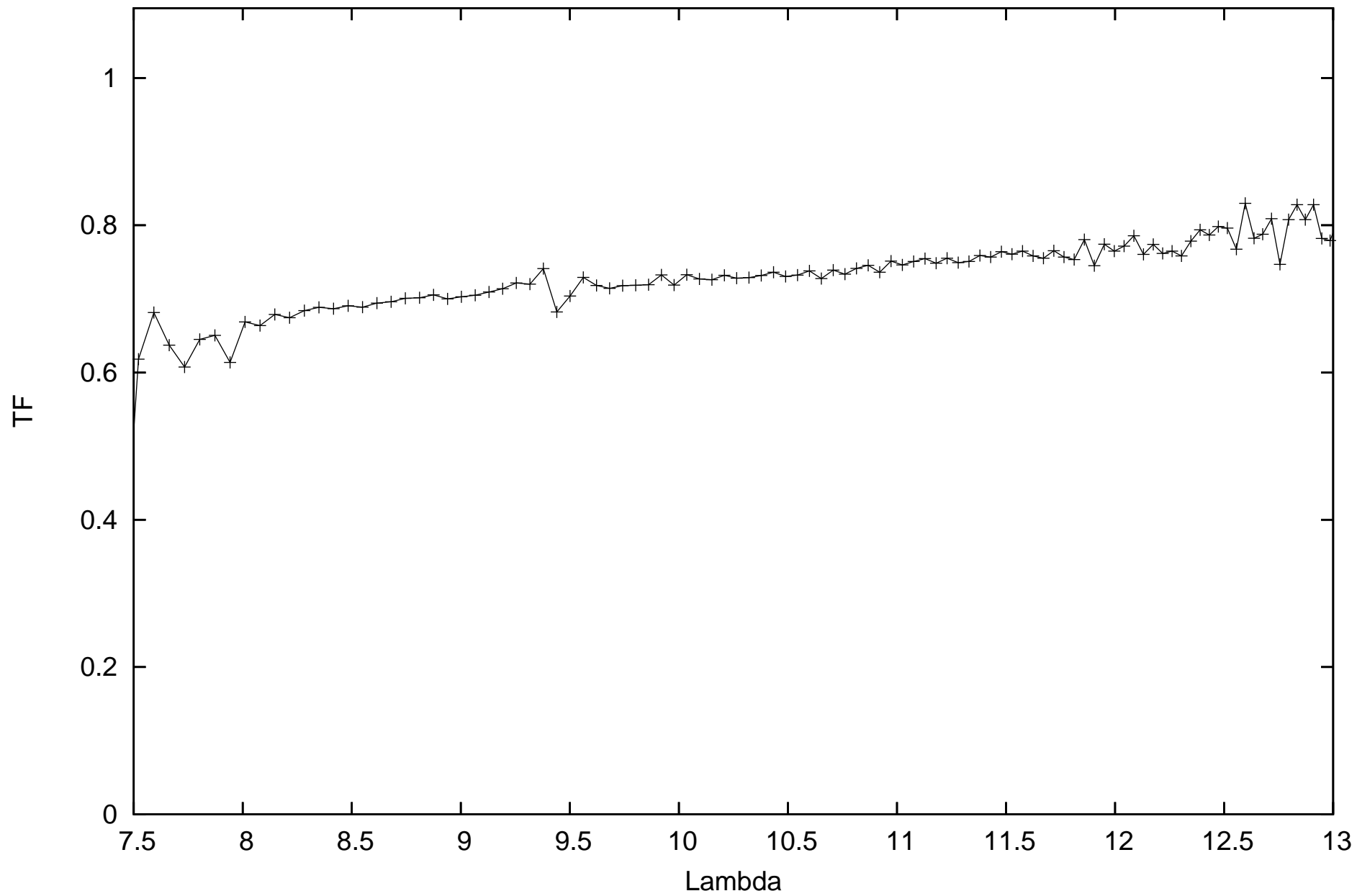
calHD167618_flux-1.82_diam11.66_r.MIDI.2009-11-03T00_58_19.000_E0G0
