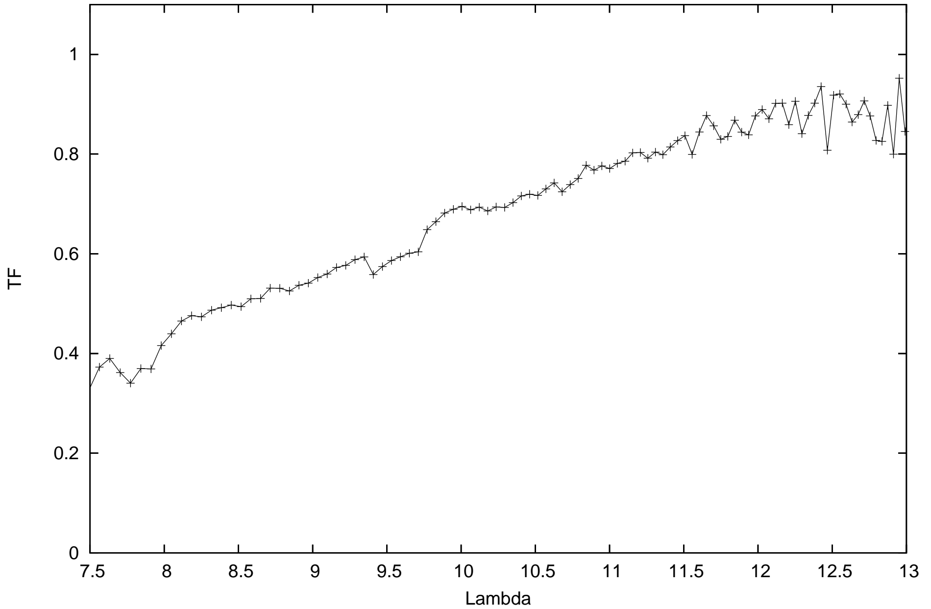
calHD167618_flux-1.82_diam11.66_r.MIDI.2009-08-15T05_41_00.110 SCIPHOT
