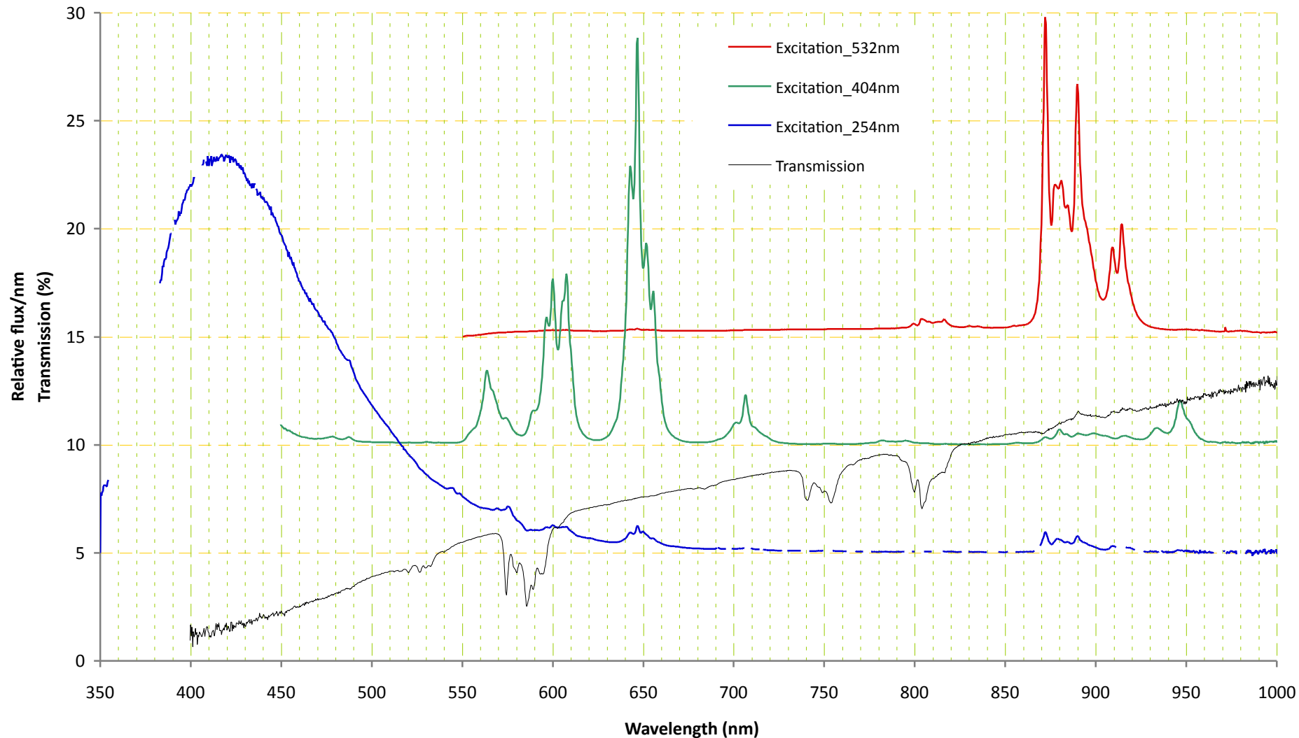
Scheelite, Italy (small sample); GB/RAEF; 9 September 2011 and 24 March 2013 Transmission and Fluorescence: excitation by laser at 532 and 404nm and Hg emission at 254nm
