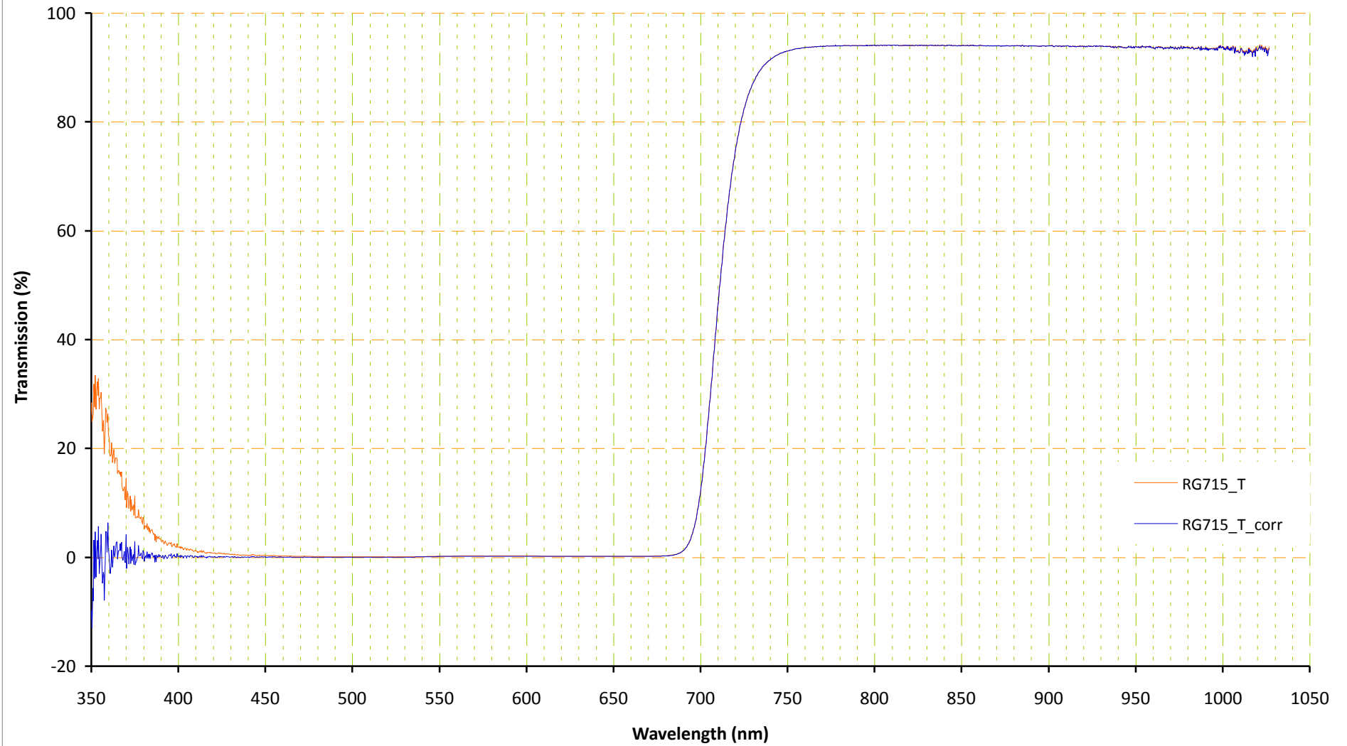
Straylight correction for a transmission measurement, Schott RG715 (3mm) 1.35 e-6 * total counts
