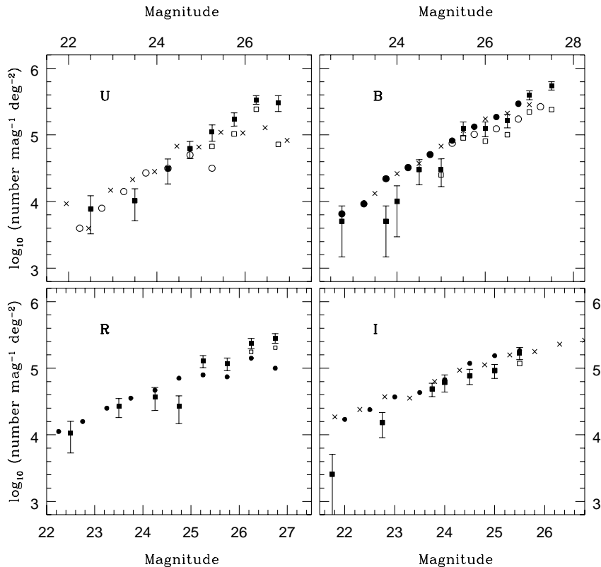
Fig. 1. Differential galaxy number counts for the U, B, R and I bands. VLT data are shown with open (raw) and filled (corrected) squares. Error bars take into account Poisson error only. Other data taken from the literature are shown. U Band : empty circles from Hogg et al 1995; crosses from HDF-N (Williams et al 1996). A correction U_J = U_{AB} - 0.8 has been applied to the latter data. B Band : (open) filled circles are (un-)corrected data from Metcalfe et al 1995. Crosses from Arnouts et al 1998. R Band : Filled circles are raw Keck data from Smail et al 1995. I Band : Filled circles are from the NTT Deep Field (Arnouts et al 1998), crosses from HDF-N (Williams et al 1996).
