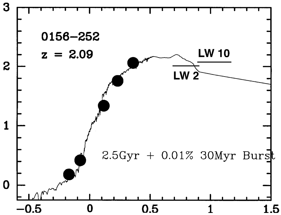
A stellar population fit to one of our sample sources observed from the ground in the optical and near-IR. The axes are logarithmic in microjanskys and microns. The expected 5-sigma limits for the CAM observations are shown.
