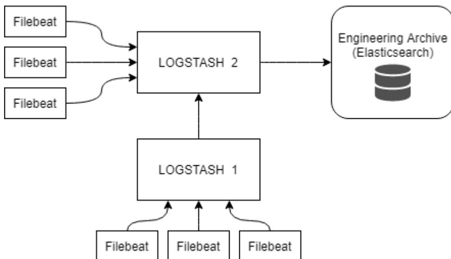
Figure 6-3 Logstash forwarding events
