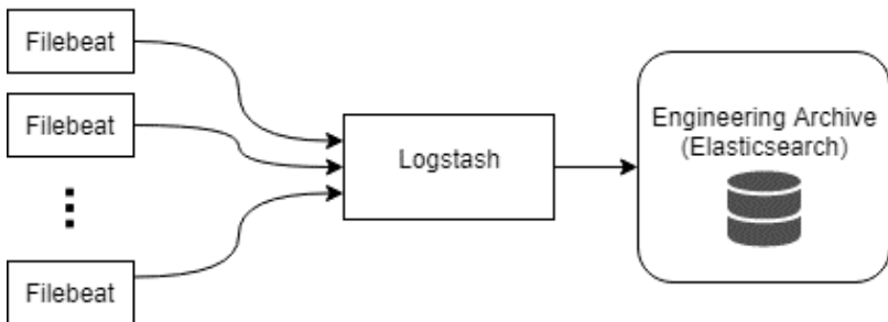
Figure 6-2 Typical log events data flow
