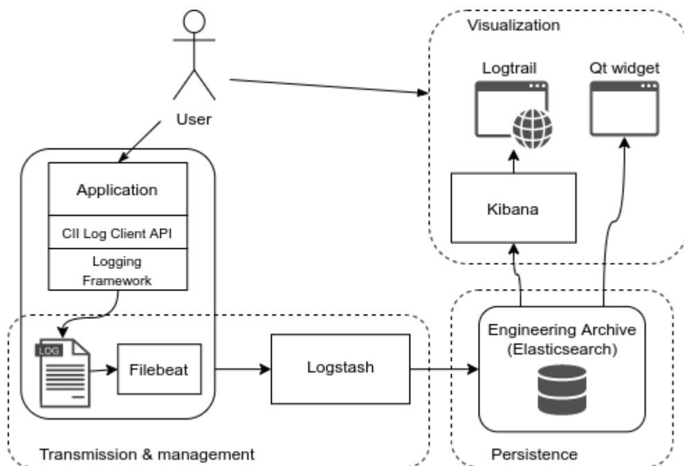
Figure 2-2 Standard workflow of CII Log system
