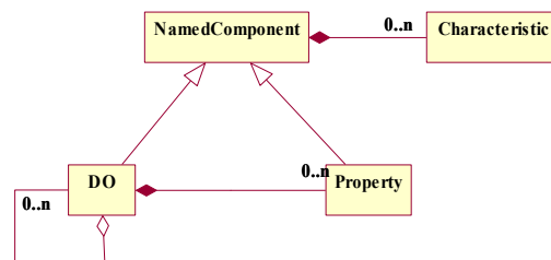
Figure 1: DO – Property – Characteristic class diagram
