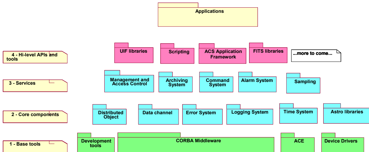
Figure 2: ACS Packages
