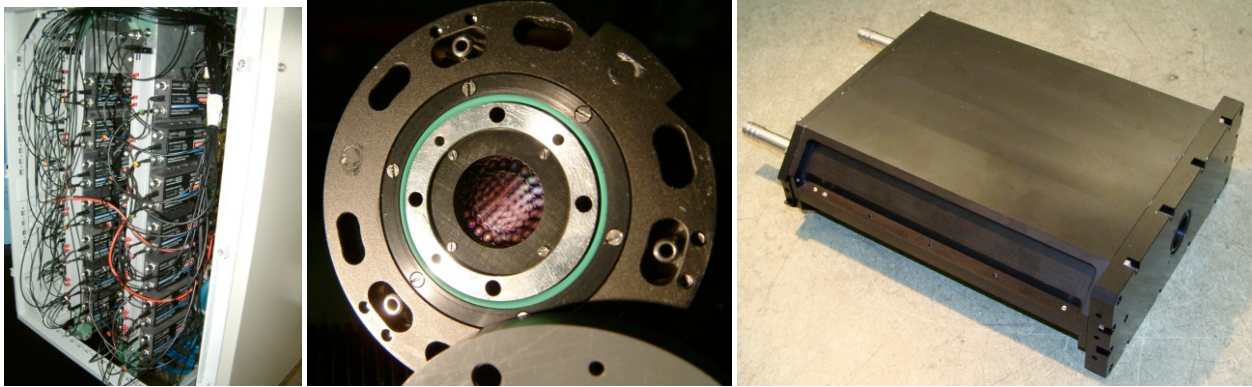
Figure 9: Three examples of line replaceable unit. From left to right: the MACAO avalanche photodiode (APD) cabinet, the MACAO lenslet array, and the Adaptive Optics Facility (AOF) wavefront sensor. The APDs are good examples of a units with a short lifetime. With more than 350 units at the observatory, the exchange frequency is almost on a weekly basis. Therefore the APDs, fibers, power plugs accessibilities and the exchange procedure have been optimized to facilitate the maintenance effort. The lenslet array and WFS provide another aspect of the LRU concept: the mounting reproducibility to avoid realignment and re-calibration of the adaptive optics system.
