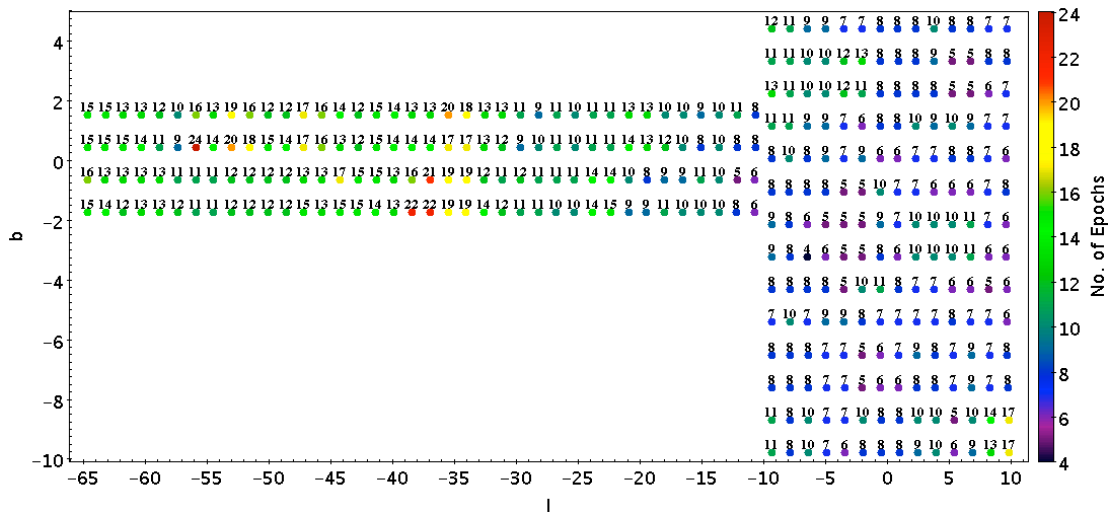
Figure 2. Colour coded plot showing the number of Ks epochs of observation for each tile in this release.
