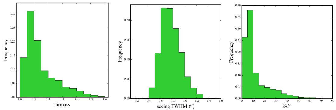
Fig 2. The left-hand and middle panels show histograms of the airmass and seeing for the observations obtained during the first two seasons of the VANDELS survey, respectively. The right-hand panel shows a histogram of the S/N ratio of the completed spectra released in DR2. The S/N ratio is measured per resolution element, in the wavelength range 6000-7400Å.
