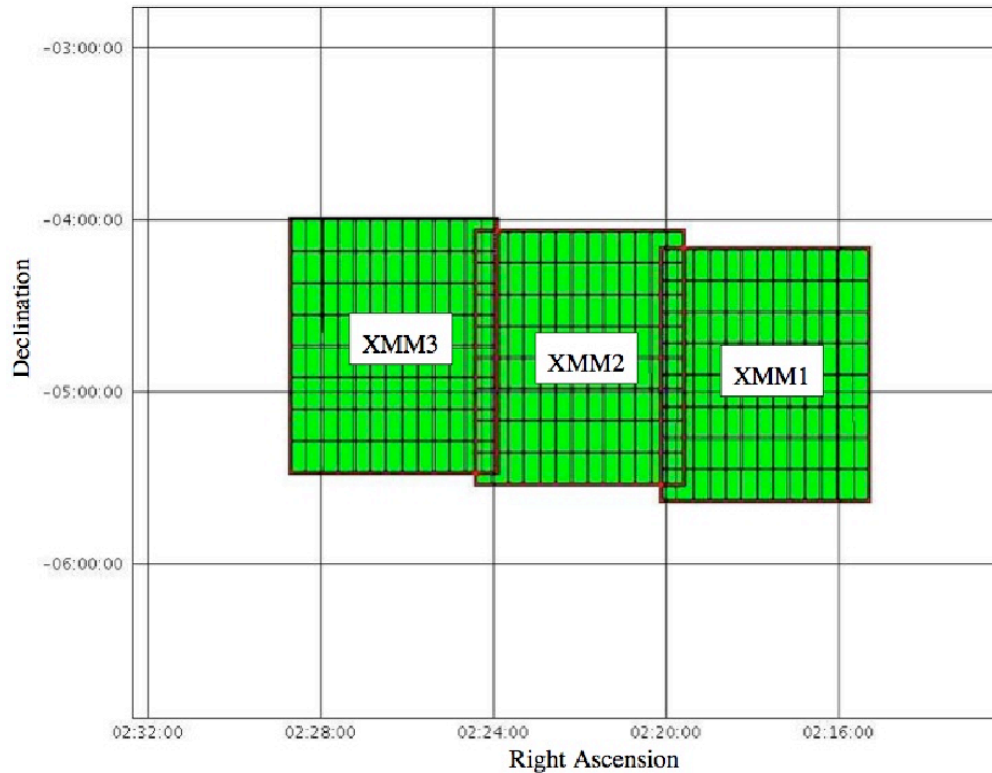
Figure. 1 The coordinates of the VIDEO-XMM field. This release comprises data over all three tiles. The deep stack data is only released over the XMM3 tile.
