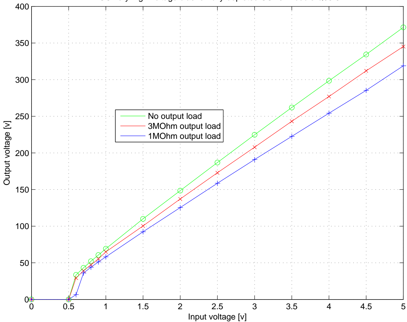
NGC very-high-voltage bias for fully-depleted CCDs. Module Q03-5.
