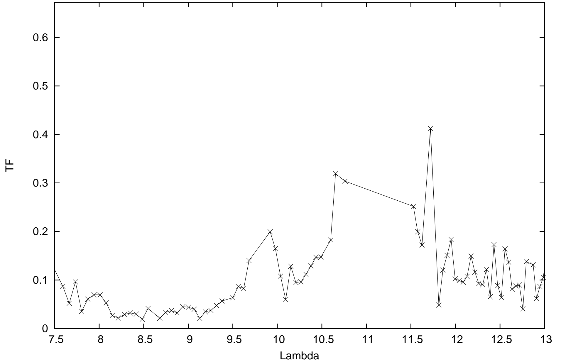
calHD81575_flux0.73_diam3.43_r.MIDI.2015-01-20T04_14_10.000_D0I1
