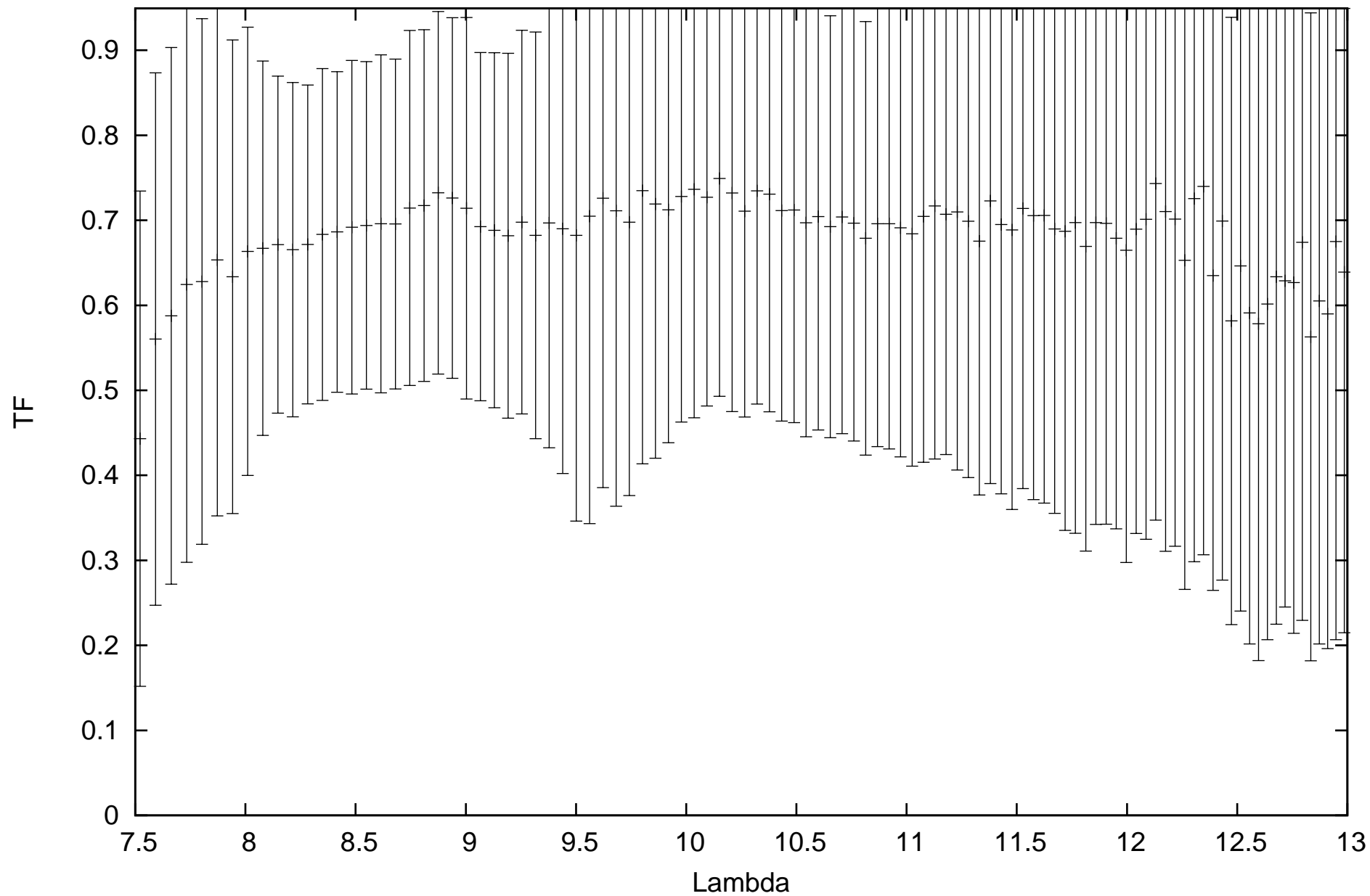
calHD65183_flux-0.08_diam5.41_r.MIDI.2015-01-21T03_28_09.000_H0G1
