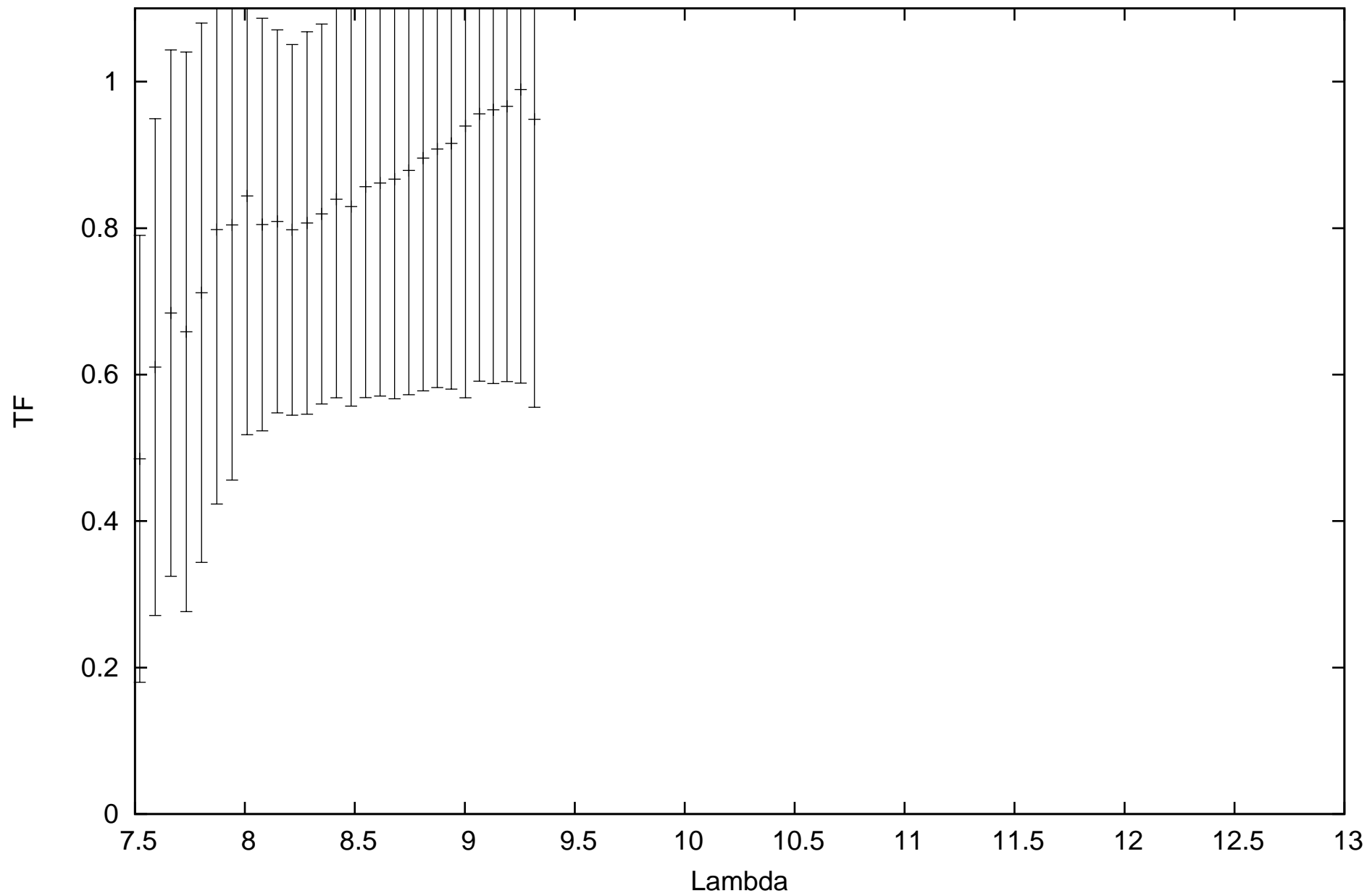
calHD54605_flux0.14_diam3.56_r.MIDI.2015-01-09T04_40_04.000_G111
