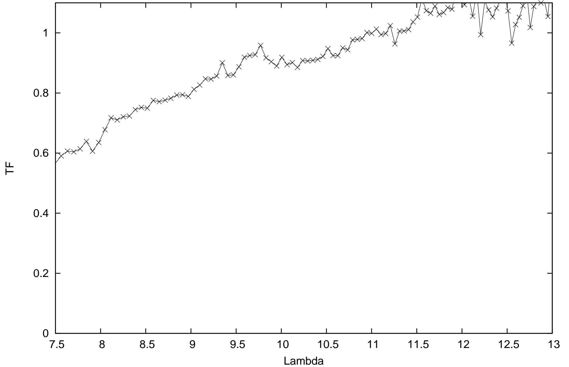
calHD48915_flux-1.39_diam6.09_r.MIDI.2015-01-19T04_47_06.112_H0G1
