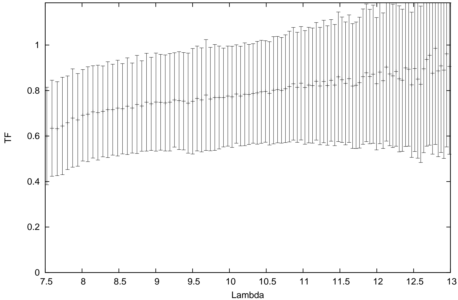
calHD48915_flux-1.39_diam6.09_r.MIDI.2015-01-09T04_23_06.000_G111
