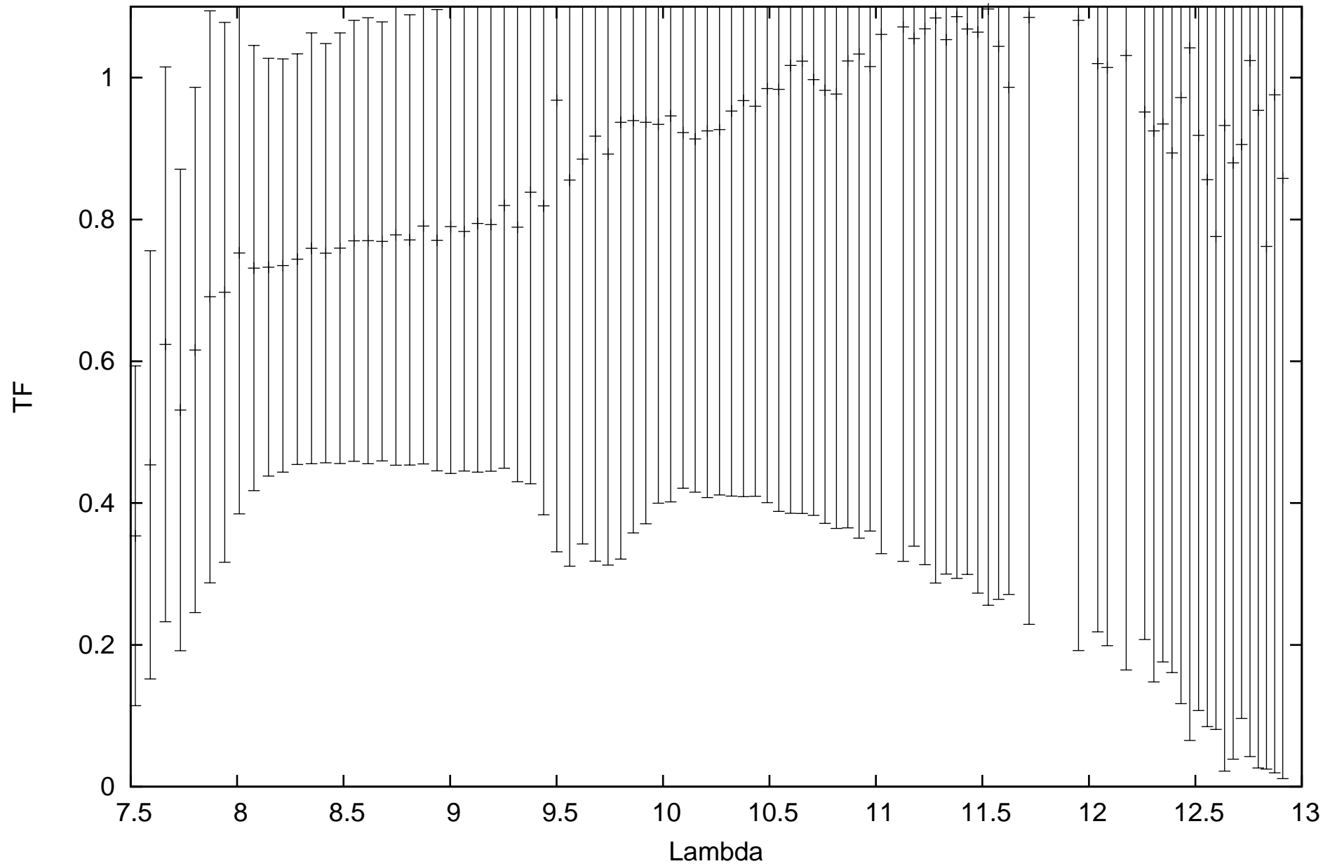
calHIP50371_flux-0.22962_diam5.18_r.MIDI.2015-01-20T04_50_56.000_D011
