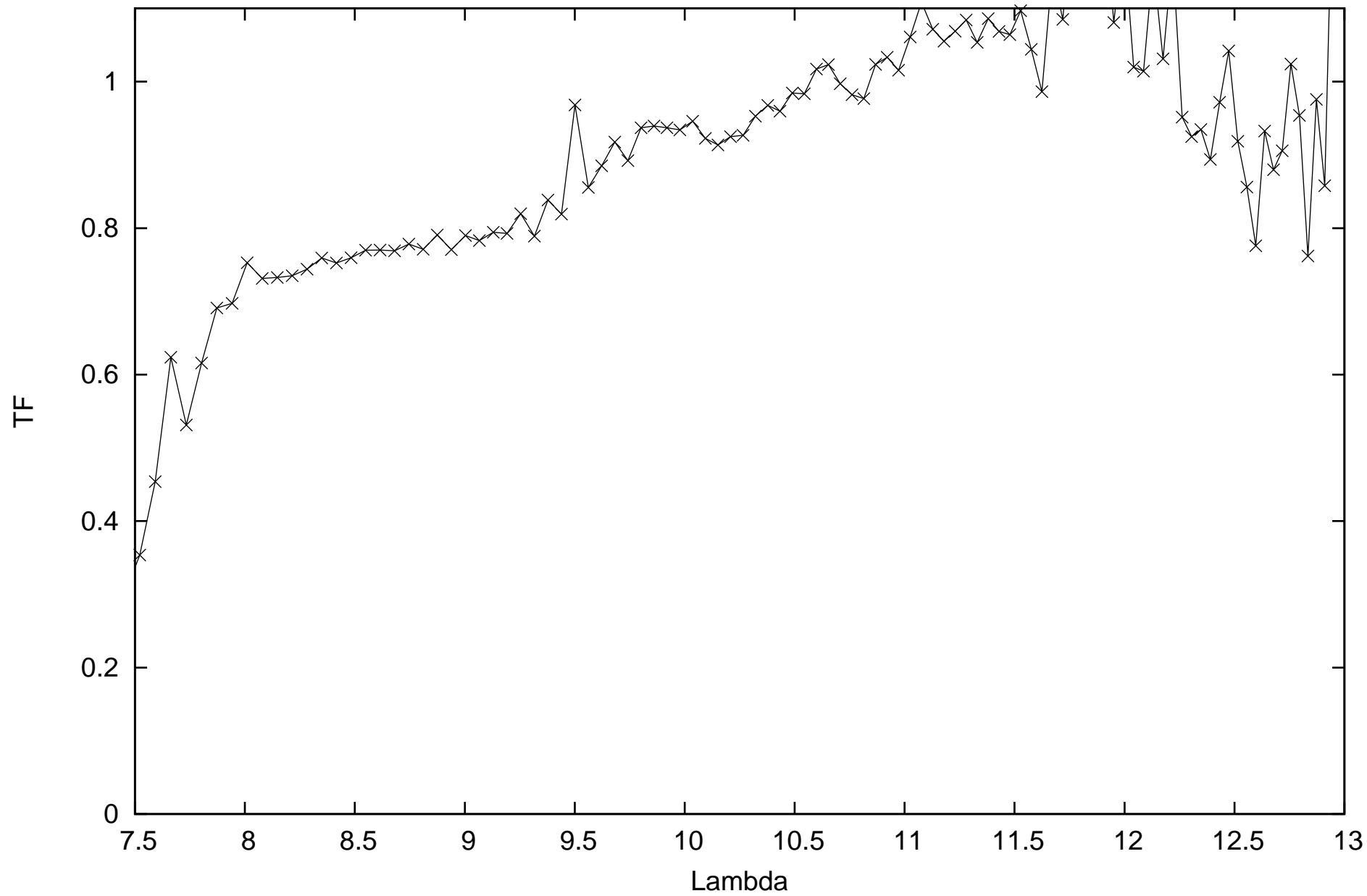
calHIP50371_flux-0.22962_diam5.18_r.MIDI.2015-01-20T04_50_56.000_D011
