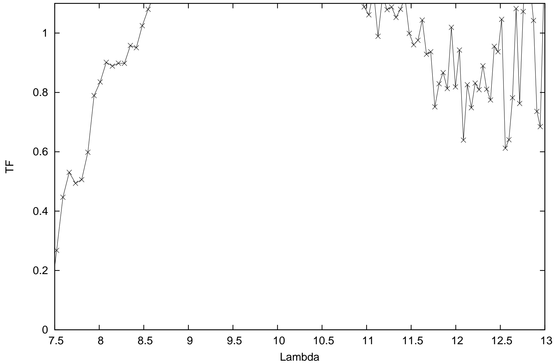
calHD81575_flux0.73_diam3.43_r.MIDI.2015-01-19T08_19_31.000_H0G1
