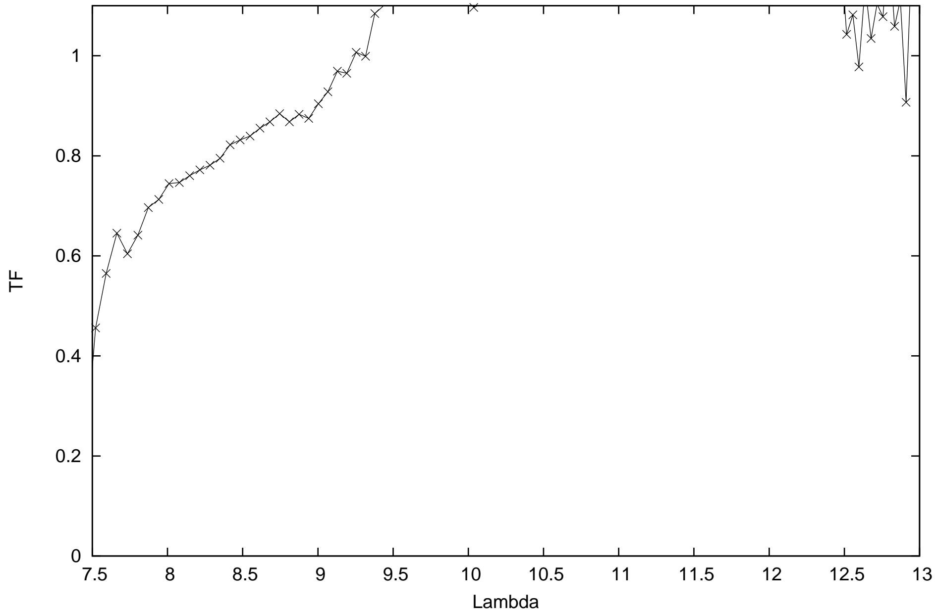
calHD65183_flux-0.08_diam5.41_r.MIDI.2015-01-19T07_47_00.000_H0G1
