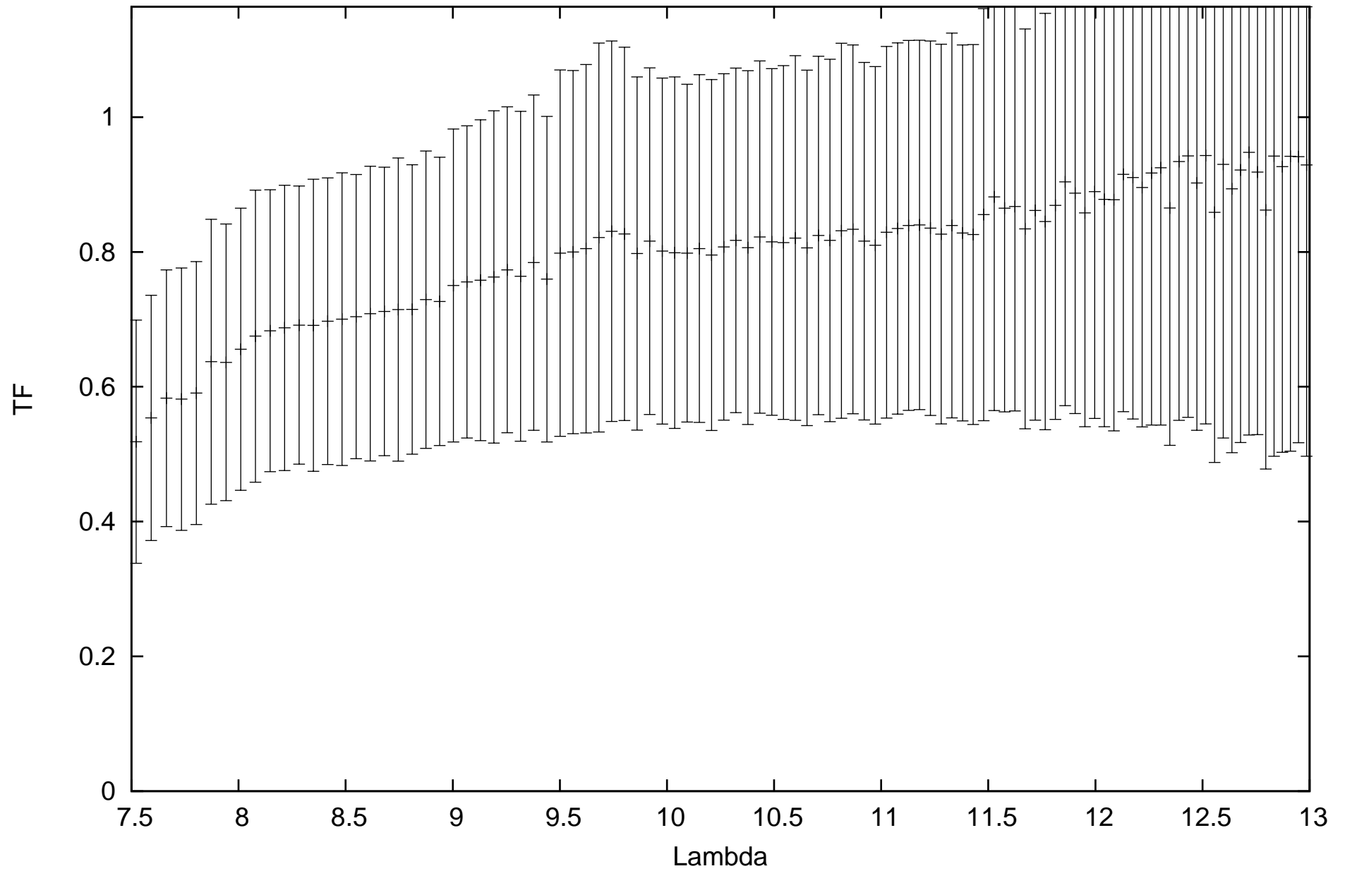
calHD81797_flux-1.49_diam9.14_r.MIDI.2015-01-18T08_07_59.000_D0H0
