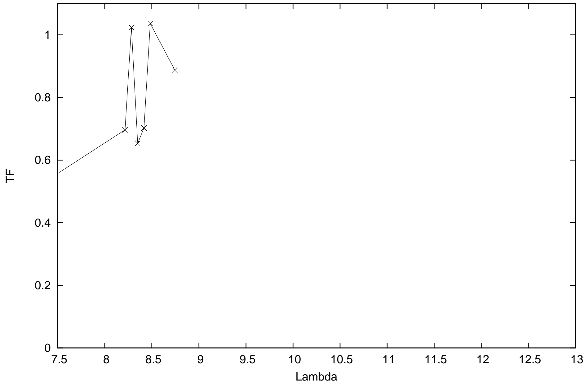
calHIP13701_flux1.17204_diam2.55_r.MIDI.2015-01-12T02_55_54.000_K0I1
