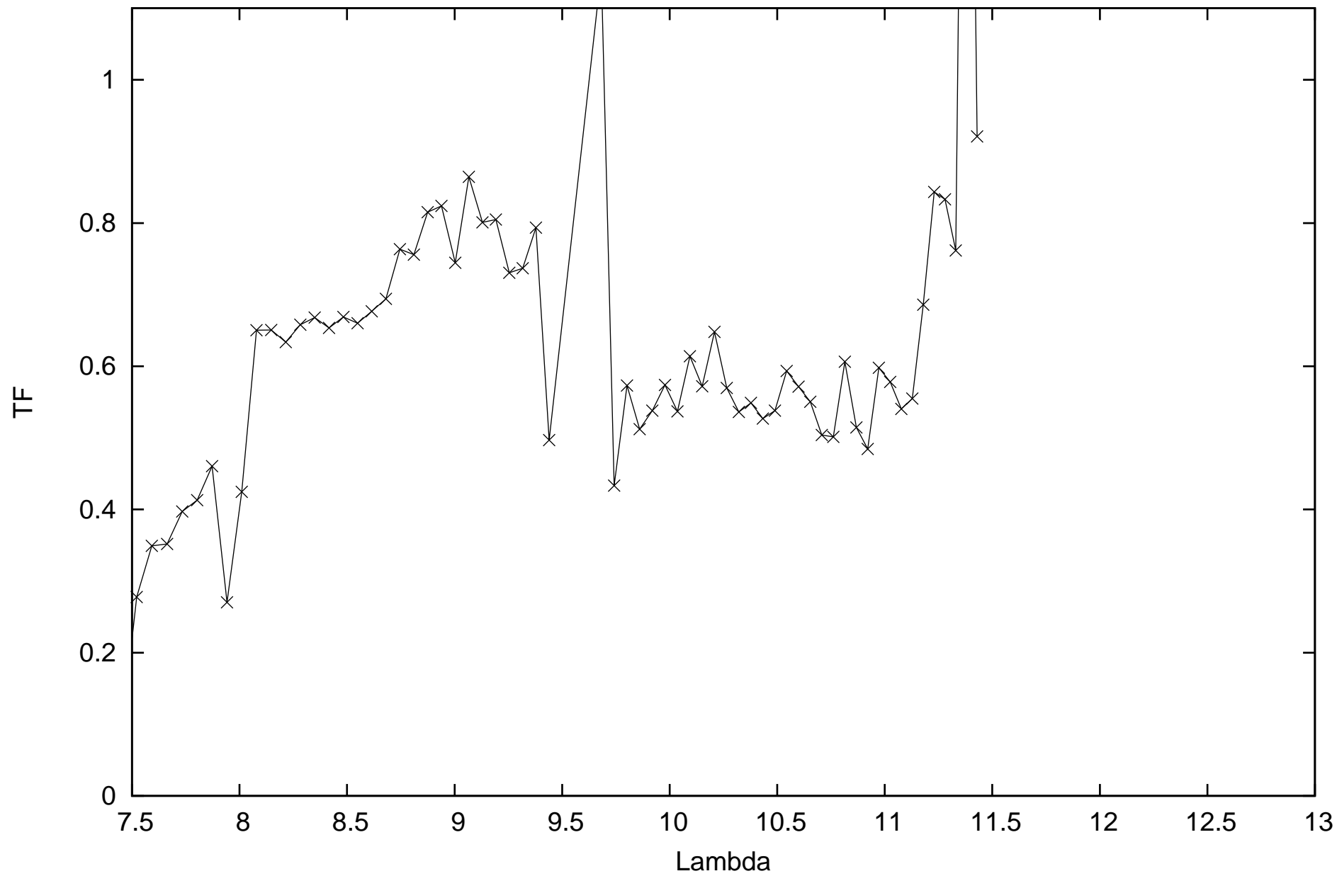
calHIP13701_flux1.17204_diam2.55_r.MIDI.2015-01-11T03_06_14.000_G111
