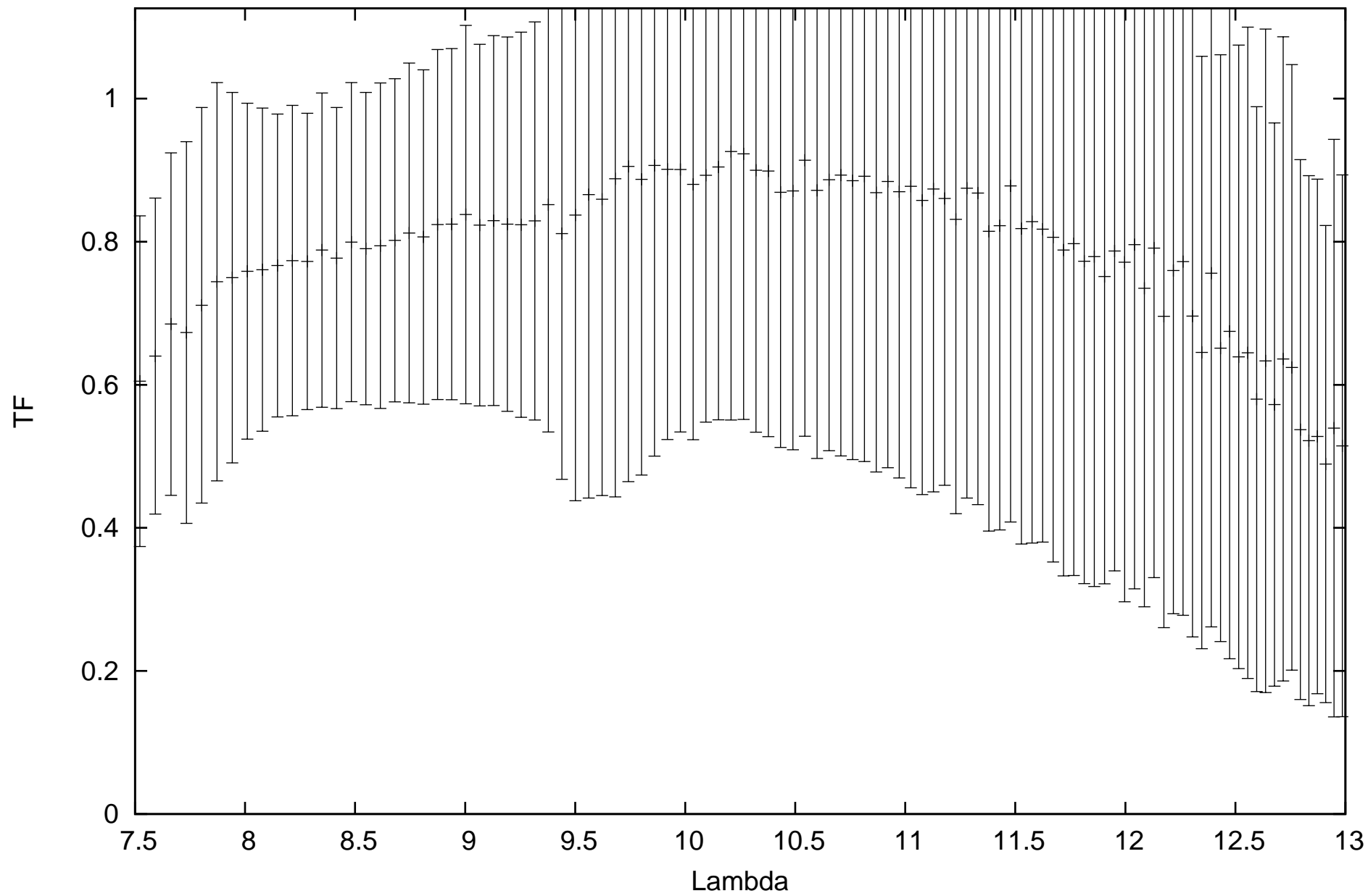
calHD54605_flux0.14_diam3.56_r.MIDI.2015-01-11T02_38_55.000_G111
