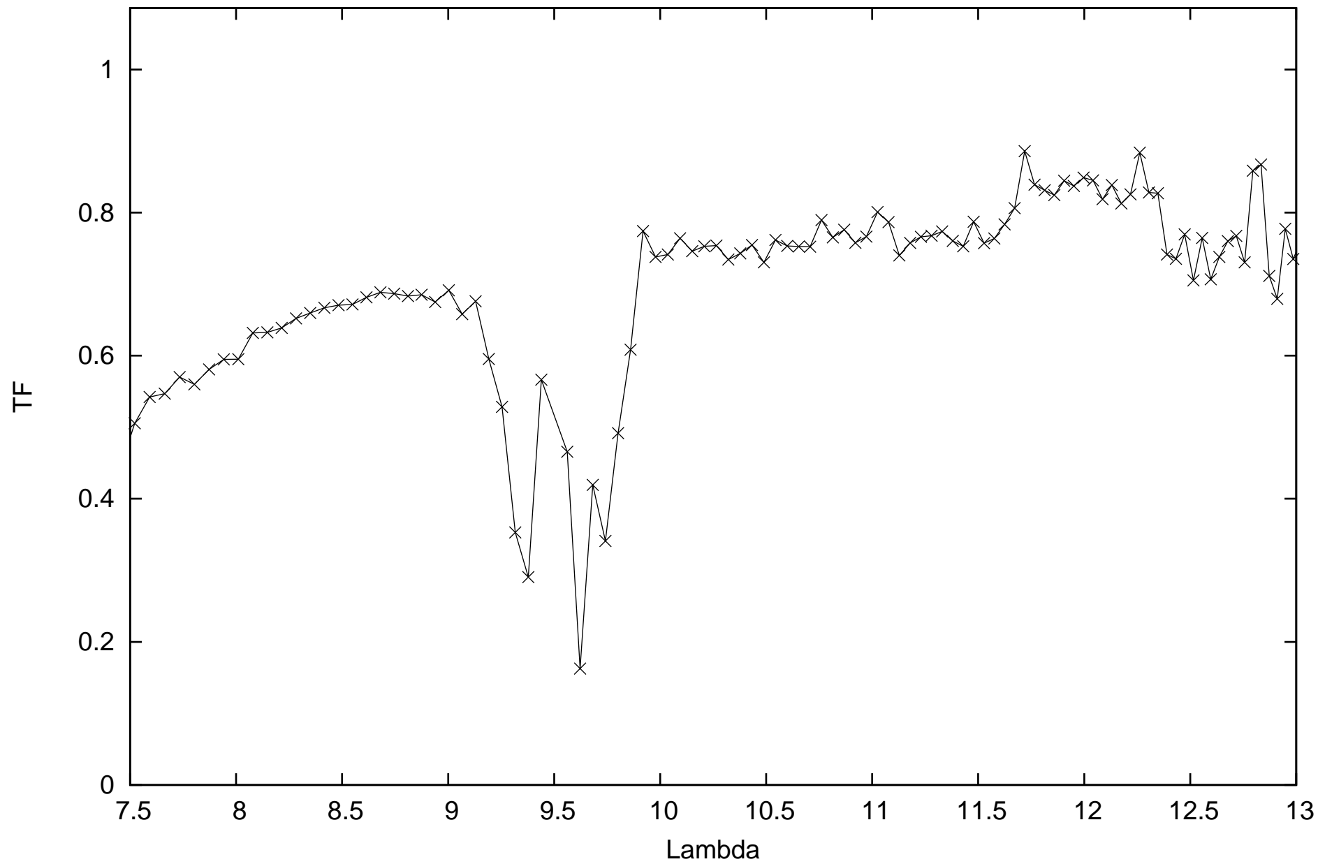
calHIP89931_flux-0.511_diam5.87_r.MIDI.2014-07-19T01_01_58.000_G1A1
