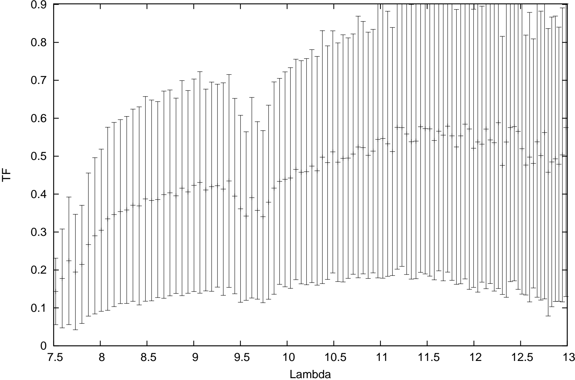
calHIP86742_flux0.007006_diam4.37_r.MIDI.2014-04-30T09_31_32.000_H011
