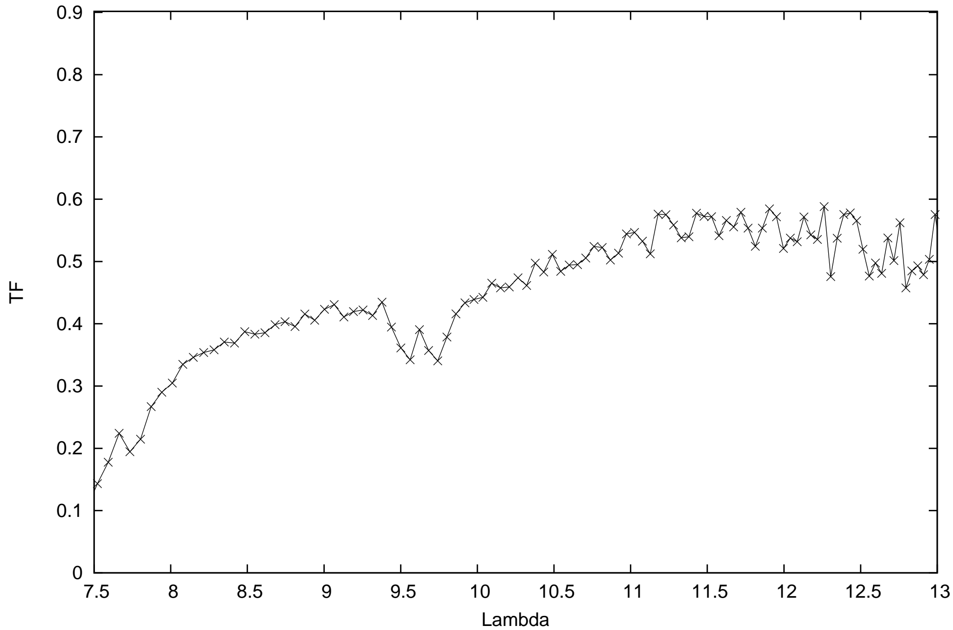
calHIP86742_flux0.007006_diam4.37_r.MIDI.2014-04-30T09_31_32.000_H011
