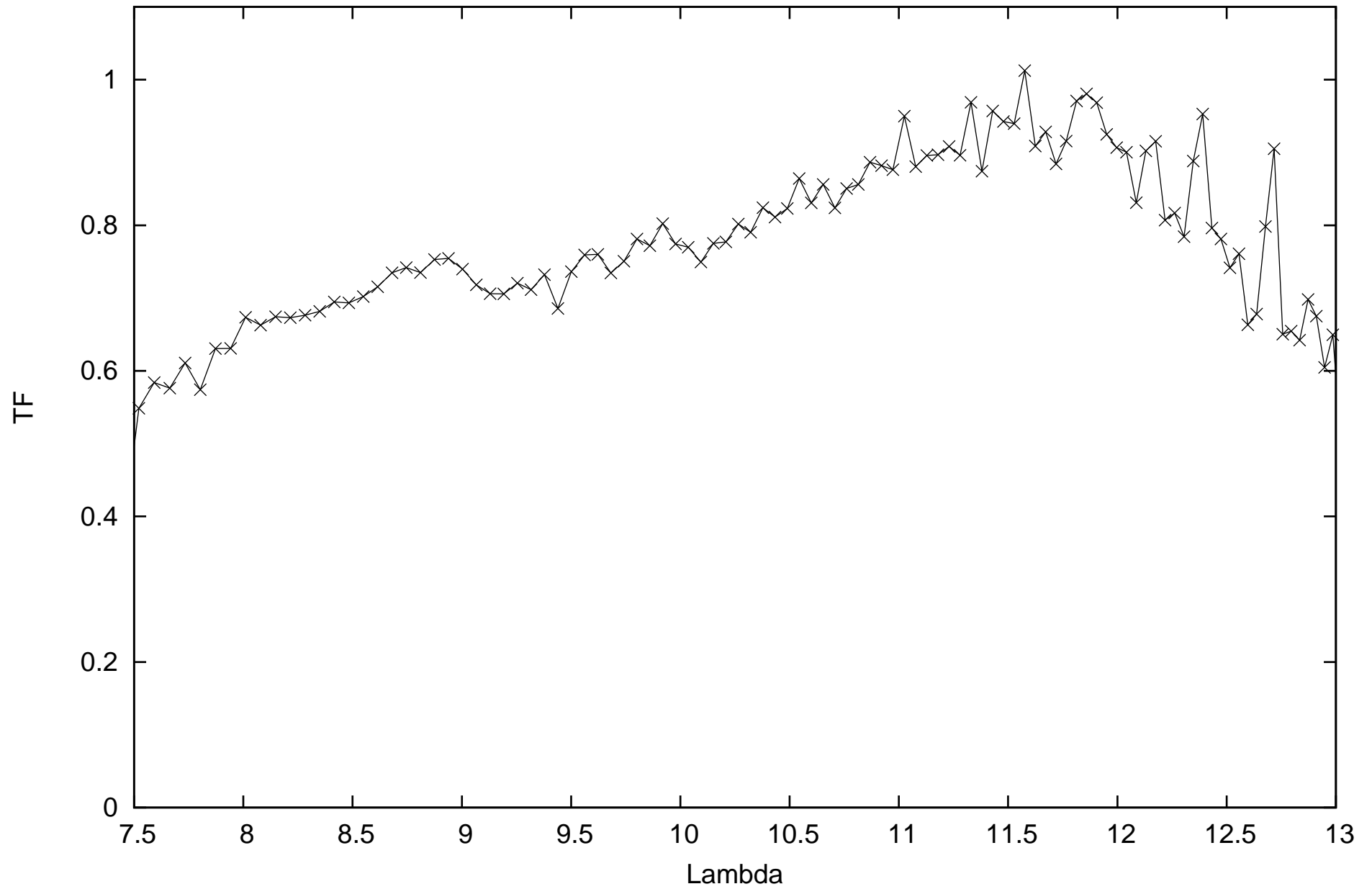
calHIP82363_flux-0.3207_diam5.52_r.MIDI.2014-07-16T01_13_43.000_G1A1
