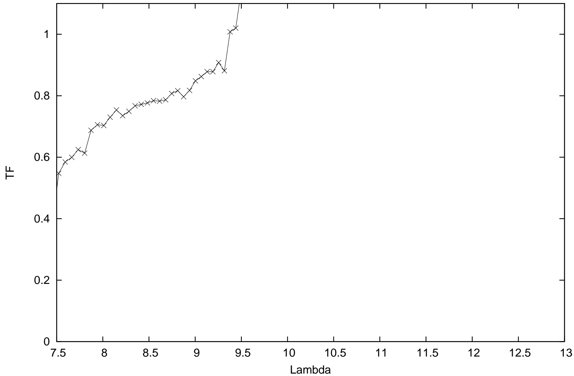
calHIP82363_flux-0.3207_diam5.52_r.MIDI.2014-06-02T04_42_44.000_C1B2
