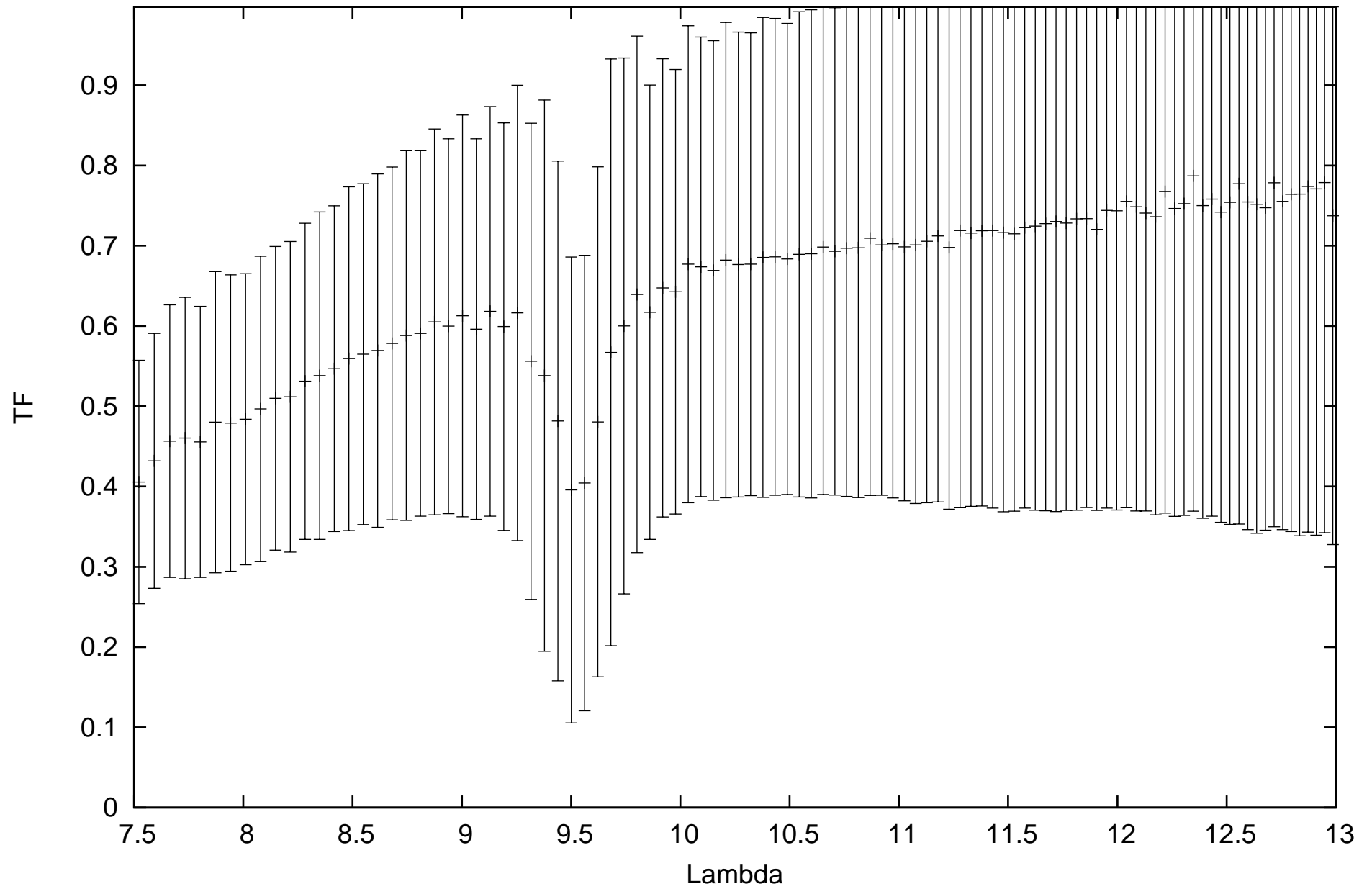
calHIP73714_flux-1.78451_diam11.15_r.MIDI.2014-07-19T00_36_48.000_G1A1
