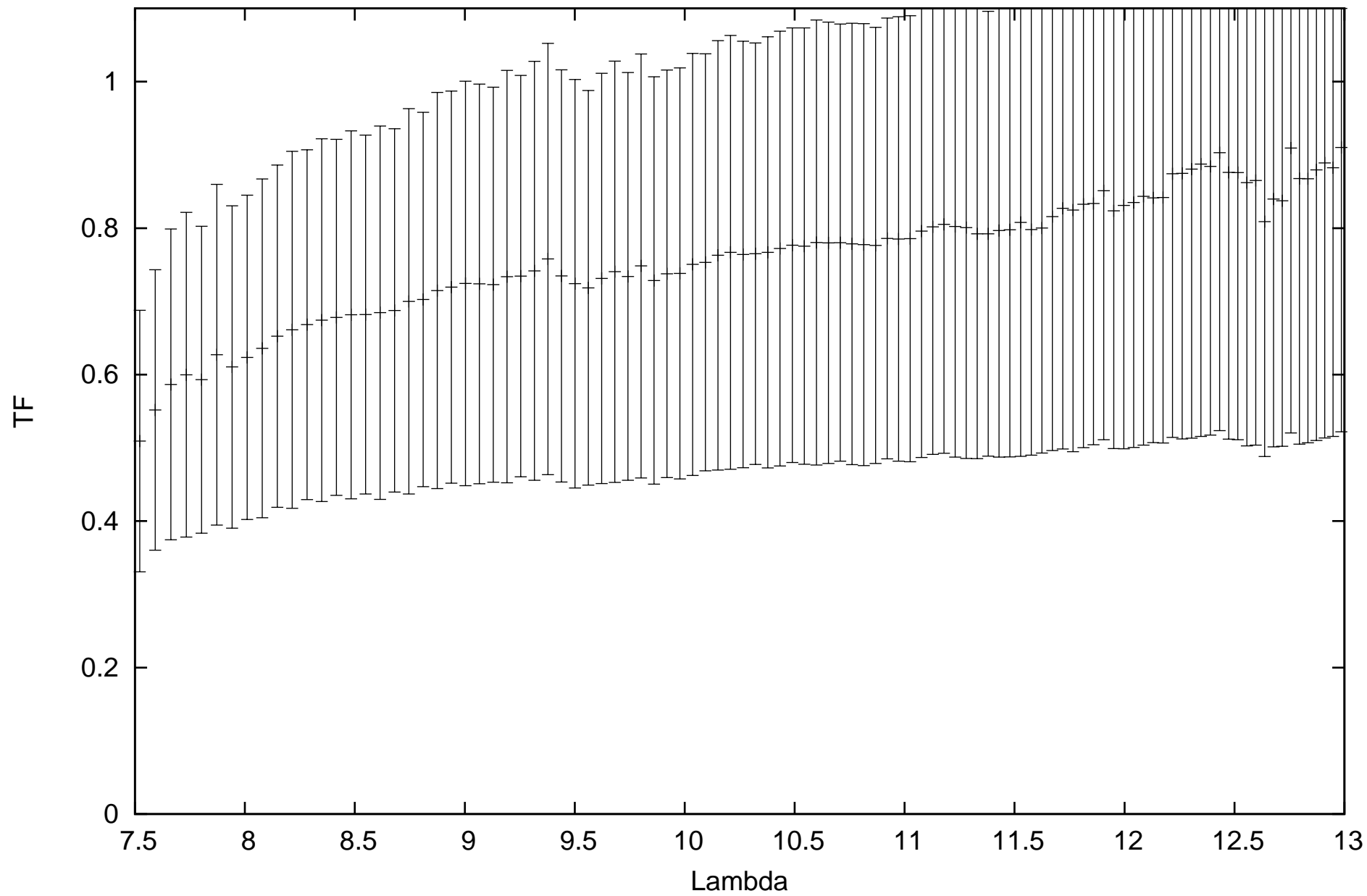
calHIP68895_flux0.550435_diam3.55_r.MIDI.2014-05-16T00_35_13.000_U1U4
