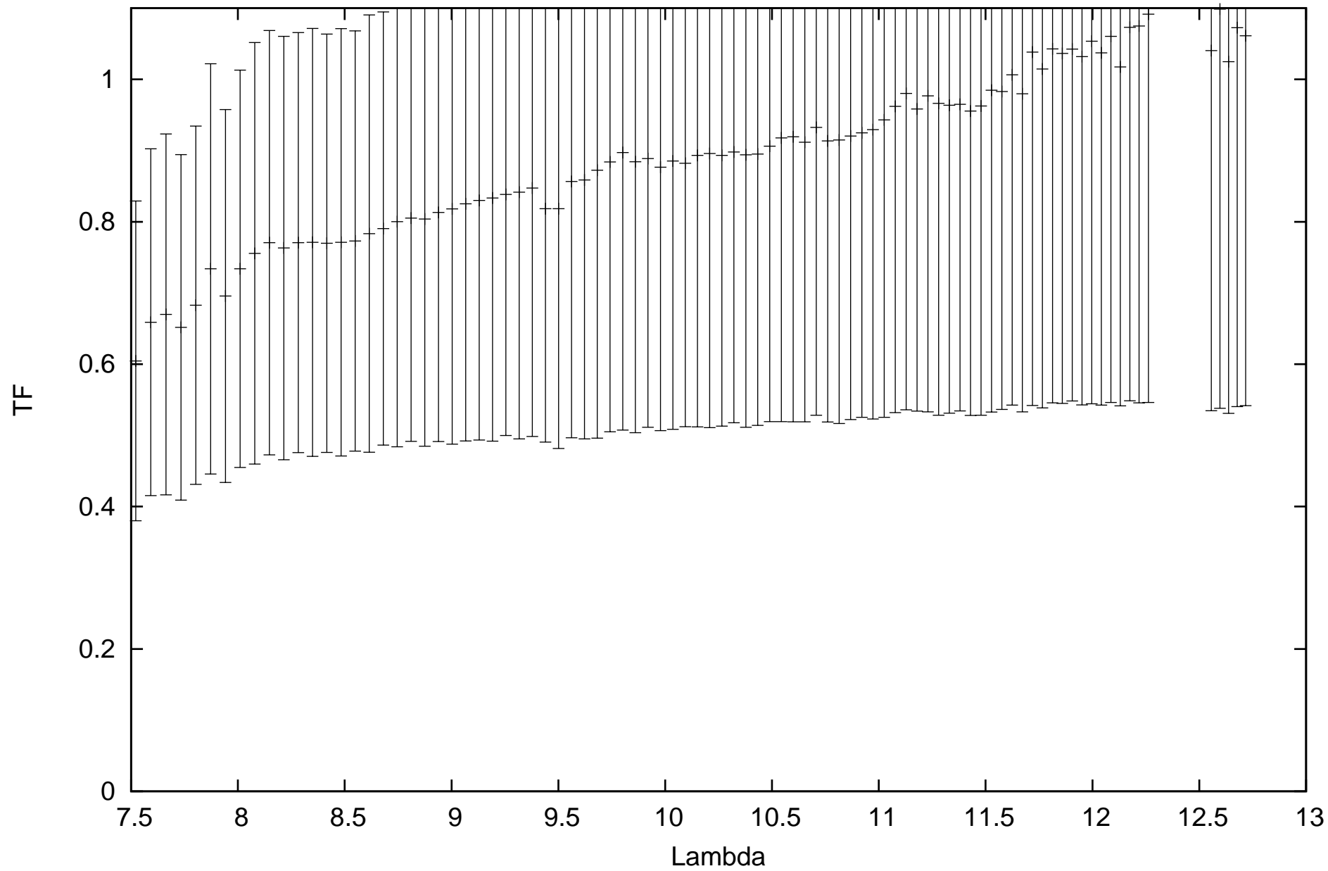
calHIP68895_flux0.550435_diam3.55_r.MIDI.2014-05-16T00_23_40.000_U1U4
