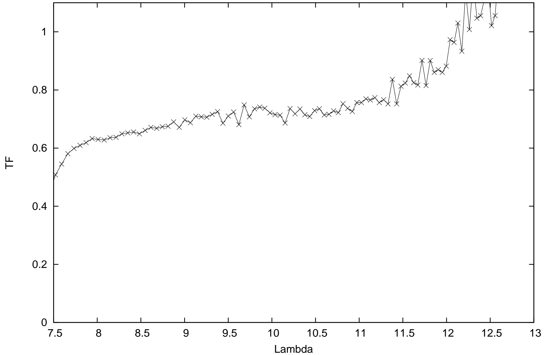
calHIP3419_flux-0.47009_diam5.23_r.MIDI.2014-12-02T02_31_55.000_G111
