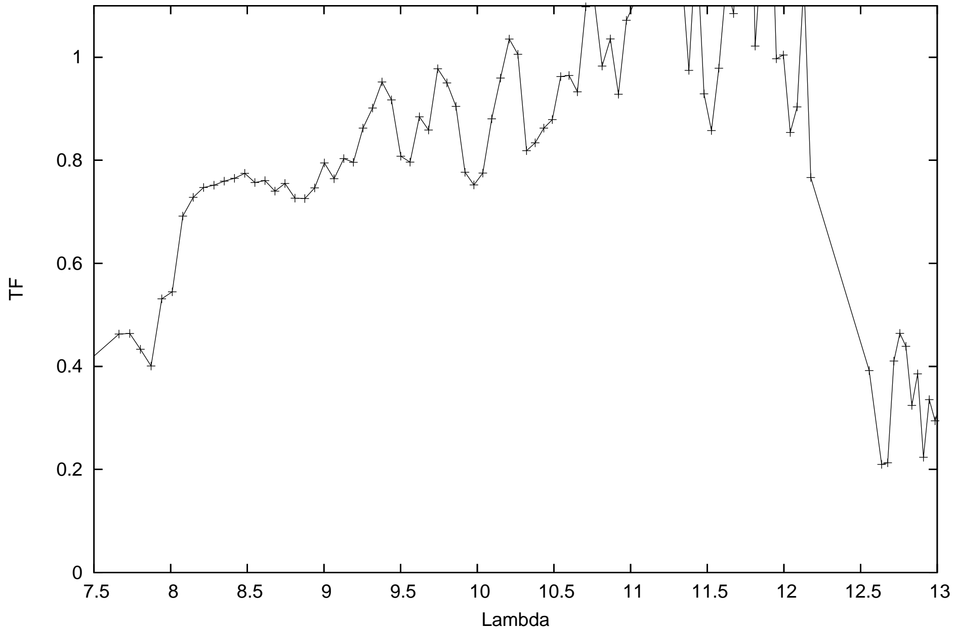
calHIP33160_flux0.496137_diam3.9_r.MIDI.2014-02-07T02_05_18.000_D0H0
