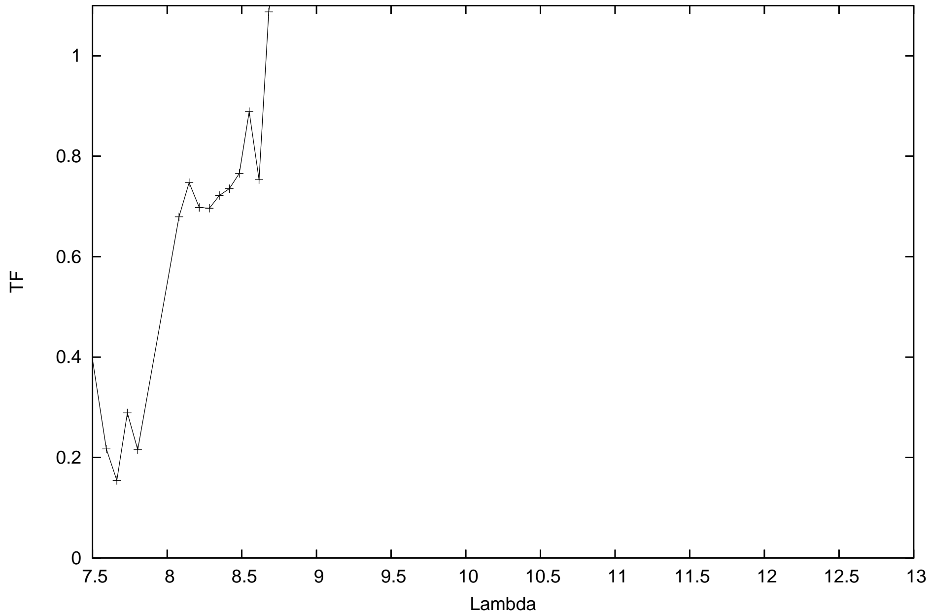
calHD98292_flux0.92_diam3.35_r.MIDI.2014-02-07T06_06_53.000_D0H0
