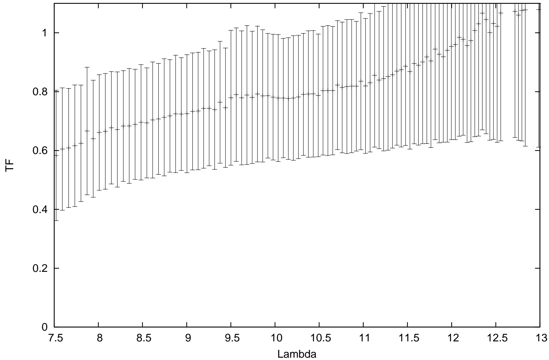
calHD81797_flux-1.49_diam9.14_r.MIDI.2014-03-27T03_19_31.000_J3K0
