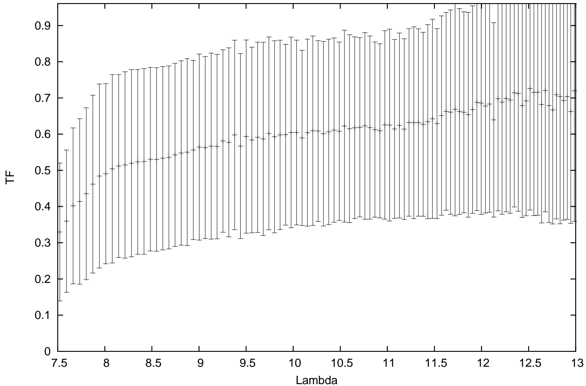
calHD81797_flux-1.49_diam9.14_r.MIDI.2014-02-19T02_43_45.000_D0H0
