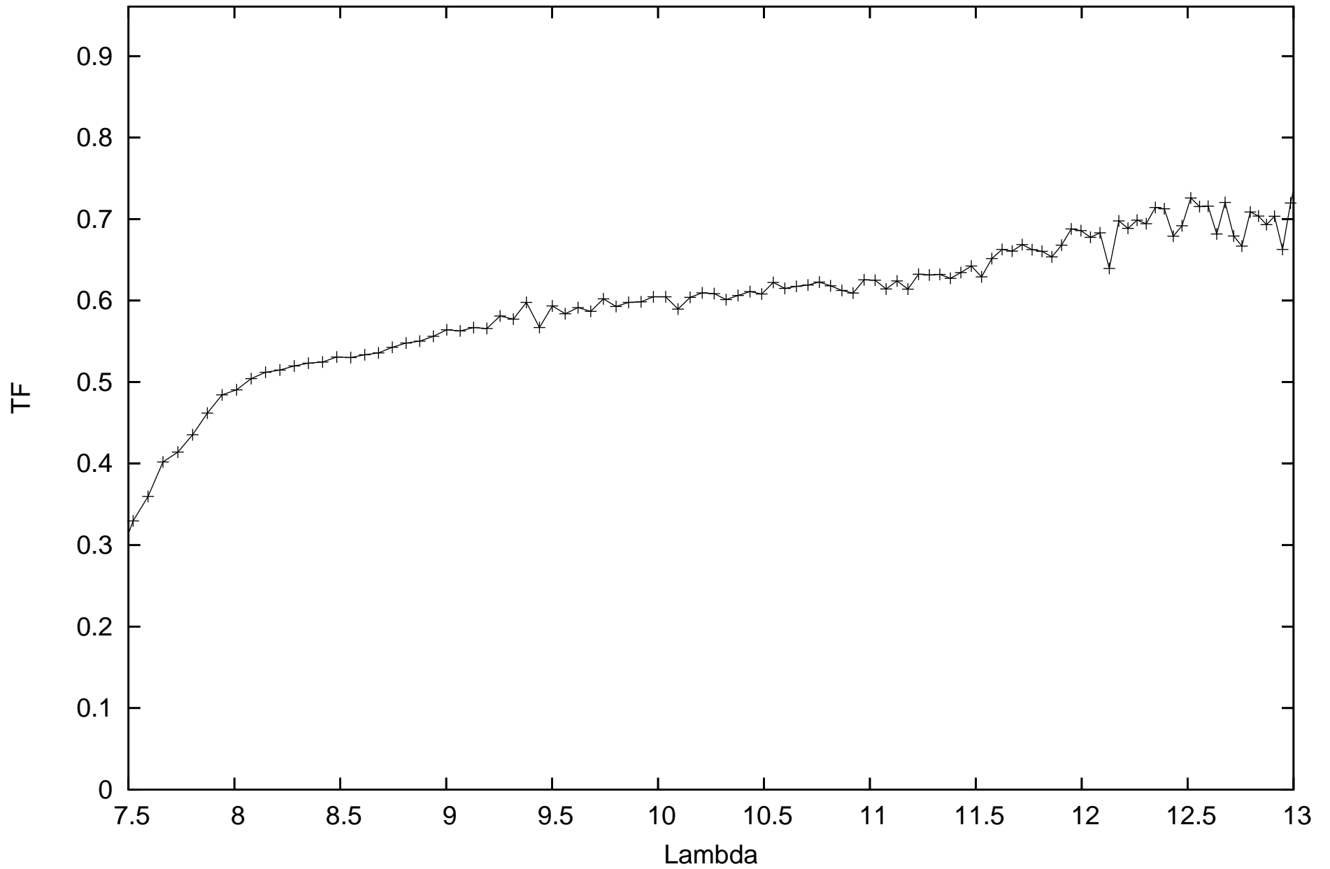
calHD81797_flux-1.49_diam9.14_r.MIDI.2014-02-19T02_43_45.000_D0H0
