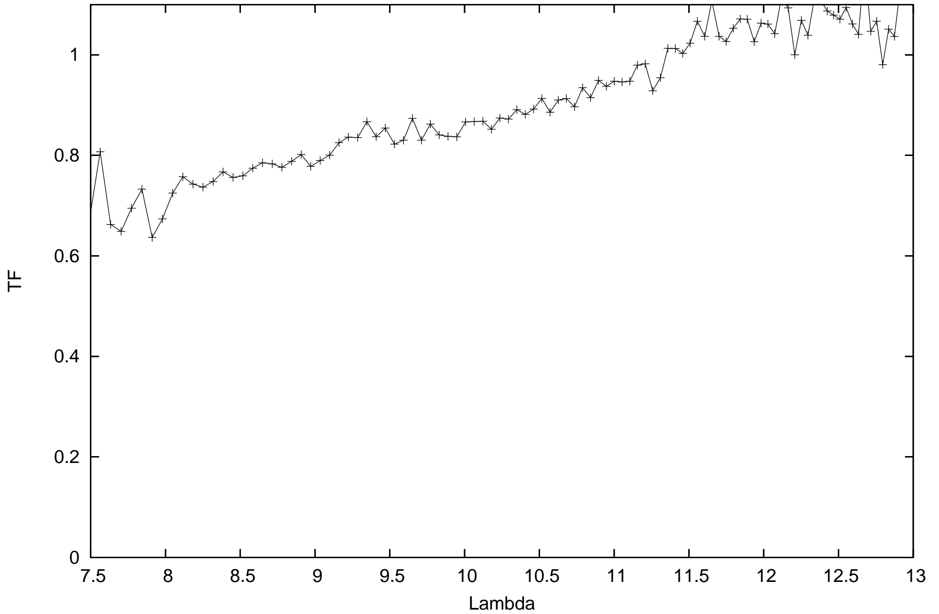
calHD81797_flux-1.49_diam9.14_r.MIDI.2014-01-11T07_37_55.135_D0B2
