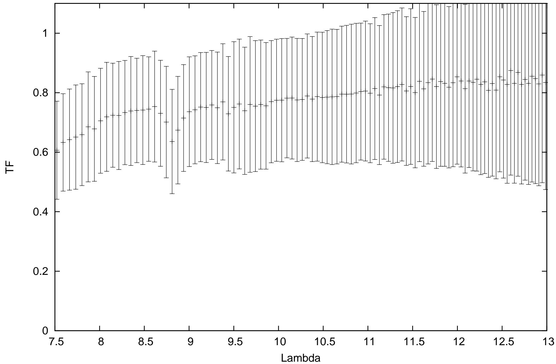
calHD48915_flux-1.39_diam6.09_r.MIDI.2014-12-26T03_35_44.000_D0B2
