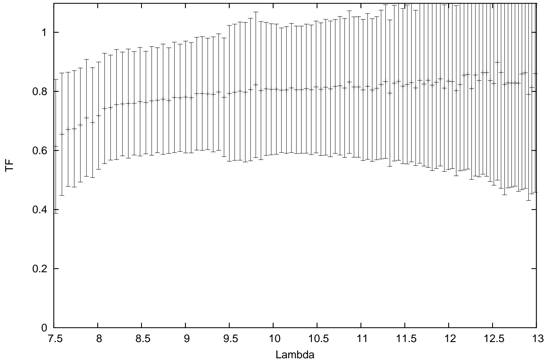
calHD48915_flux-1.39_diam6.09_r.MIDI.2014-02-09T01_47_41.000_B2A1
