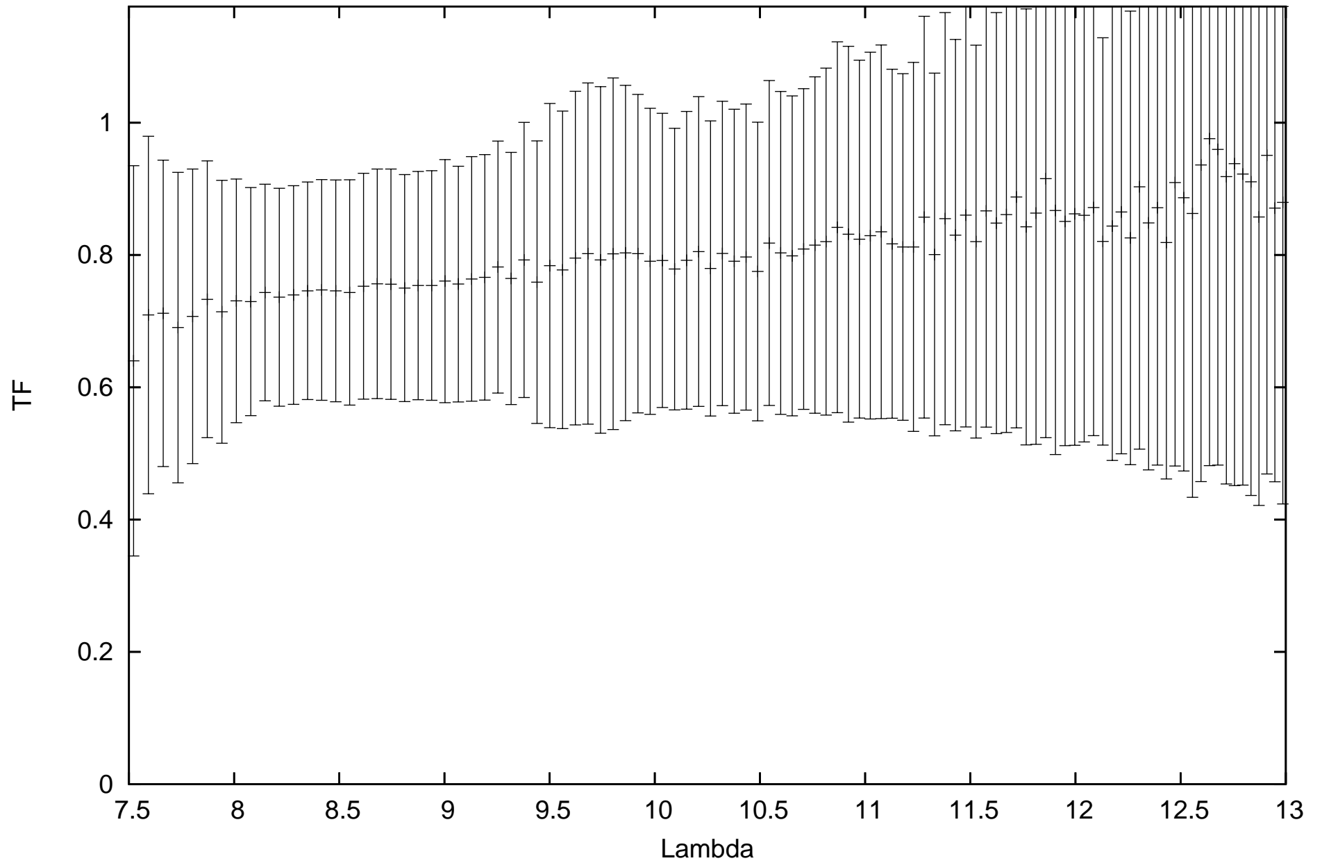
calHD48915_flux-1.39_diam6.09_r.MIDI.2014-02-04T03_28_03.000_H011
